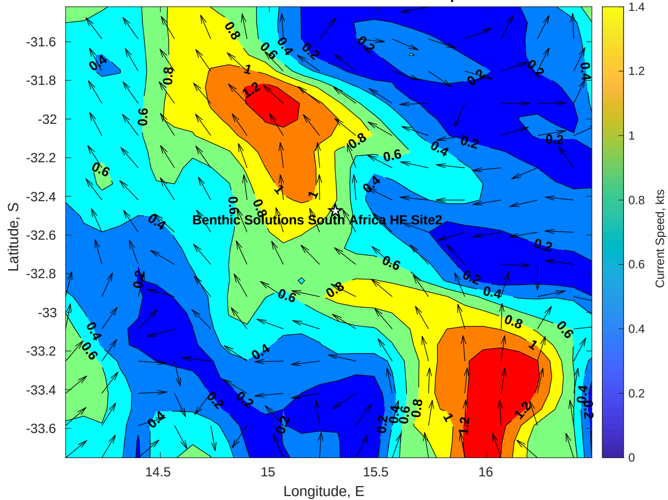
Surface Currents for Benthic Solutions South Africa HF Site2 at 14-Apr-2025 00:00:00
