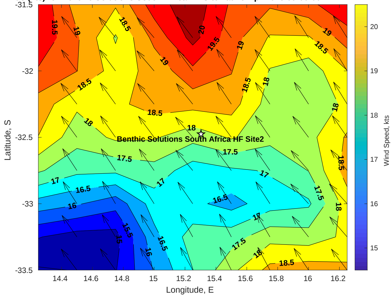
Winds (kts) for Benthic Solutions South Africa HF Site2 at 15-Apr-2025 09:00:00
