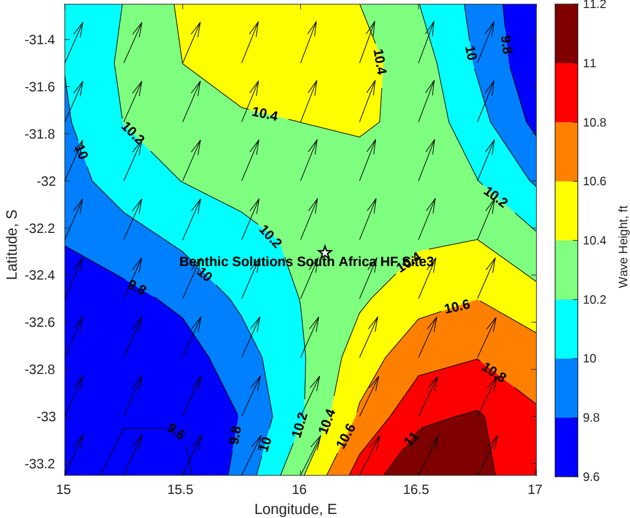
Wave Height (ft) for Benthic Solutions South Africa HF Site3 at 15-Apr-2025 09:00:00
