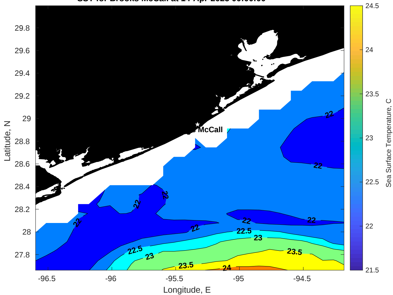
SST for Brooks McCall at 14-Apr-2025 00:00:00
