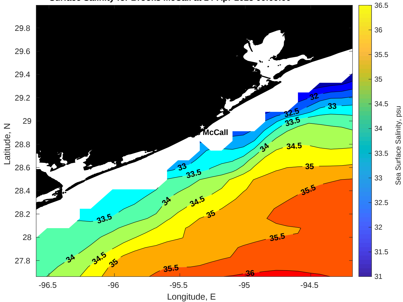
Surface Salinity for Brooks McCall at 14-Apr-2025 00:00:00
