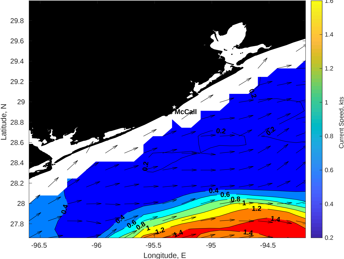
Surface Currents for Brooks McCall at 14-Apr-2025 00:00:00
