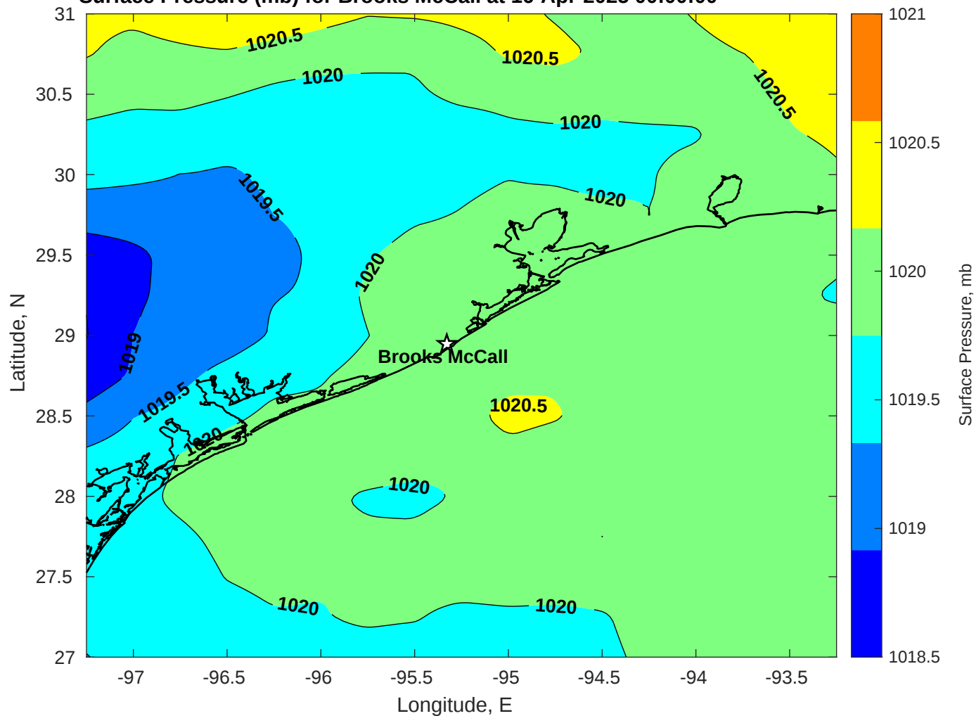
Surface Pressure (mb) for Brooks McCall at 16-Apr-2025 00:00:00
