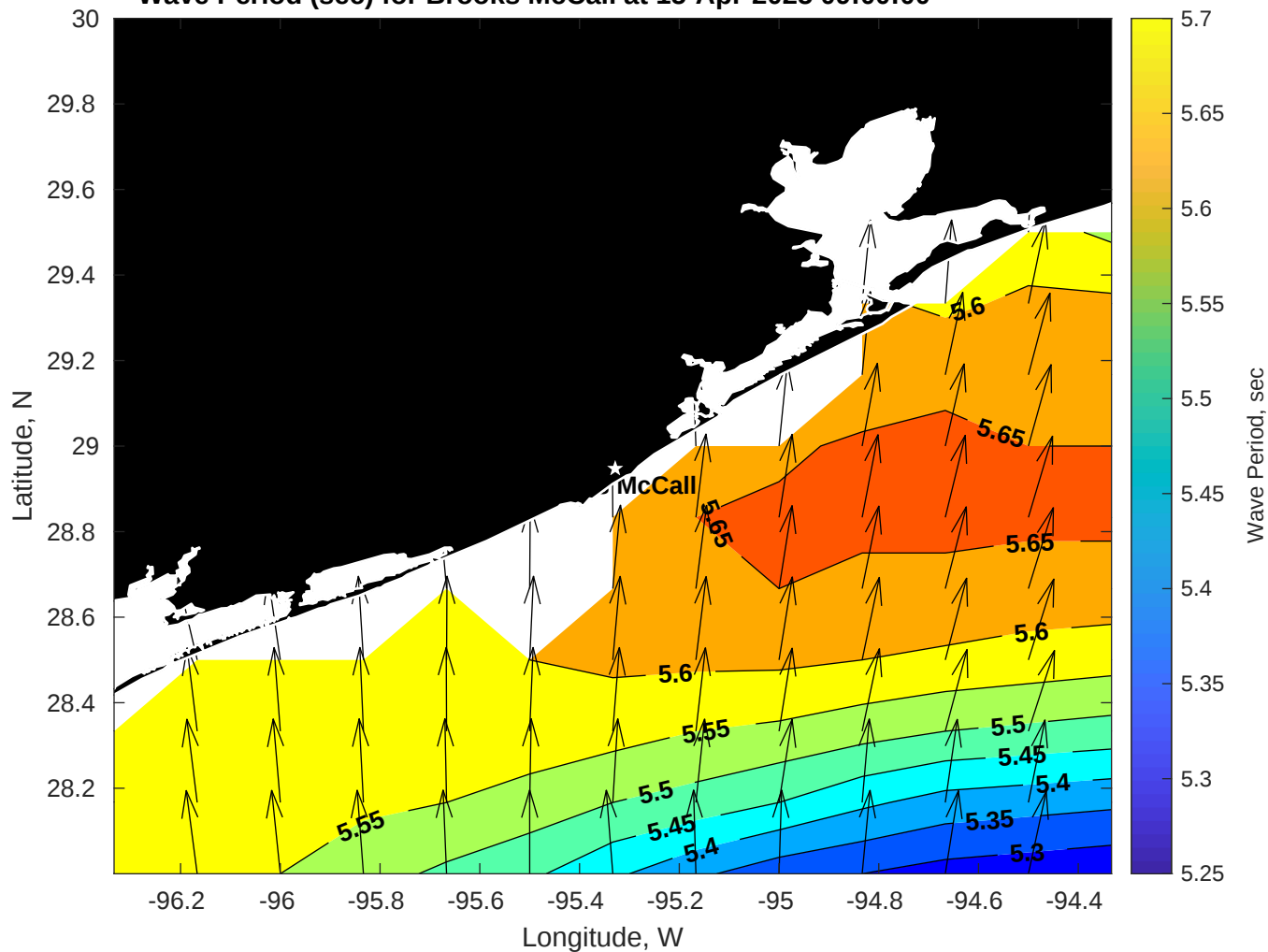
Wave Period (sec) for Brooks McCall at 15-Apr-2025 09:00:00
