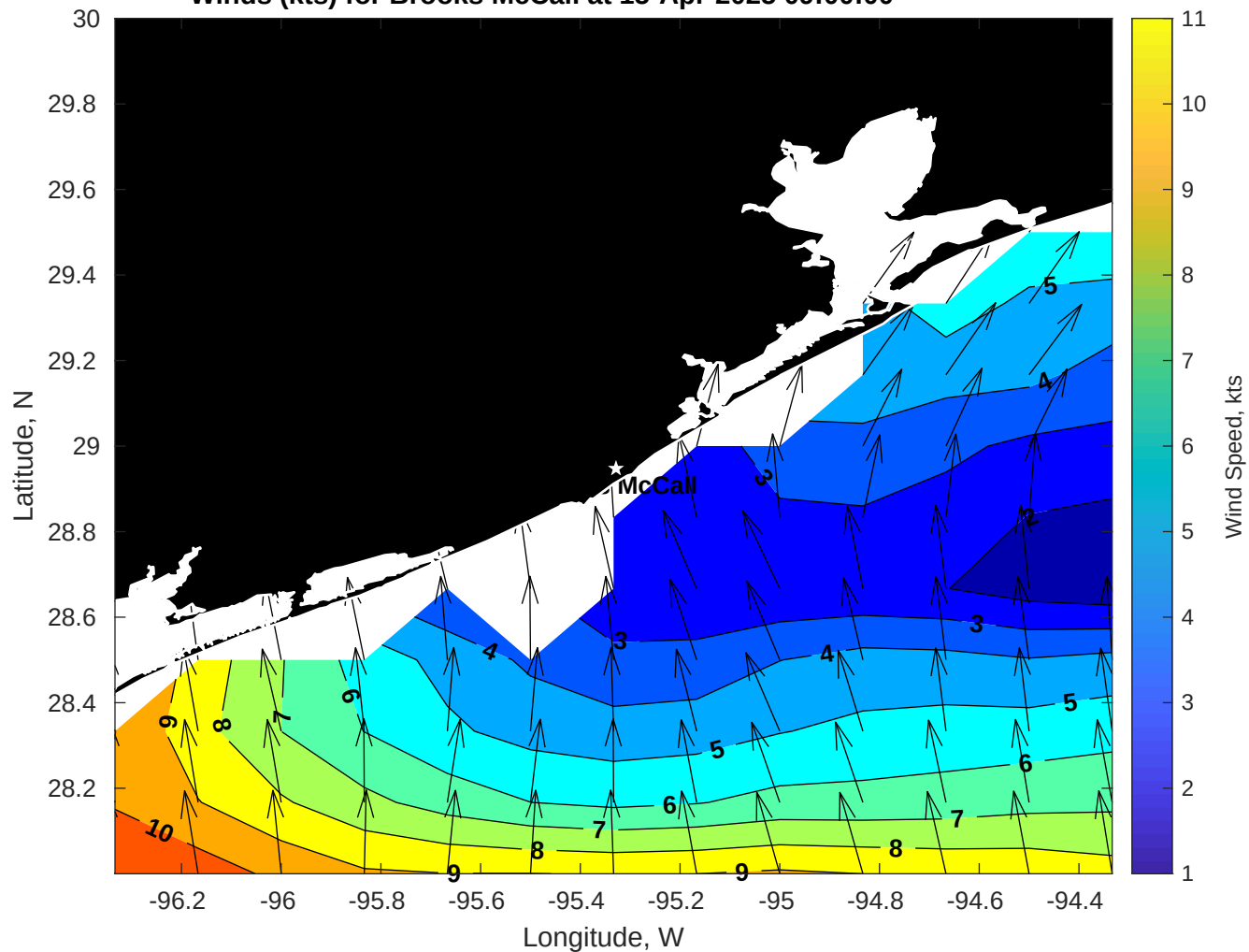
Winds (kts) for Brooks McCall at 15-Apr-2025 09:00:00
