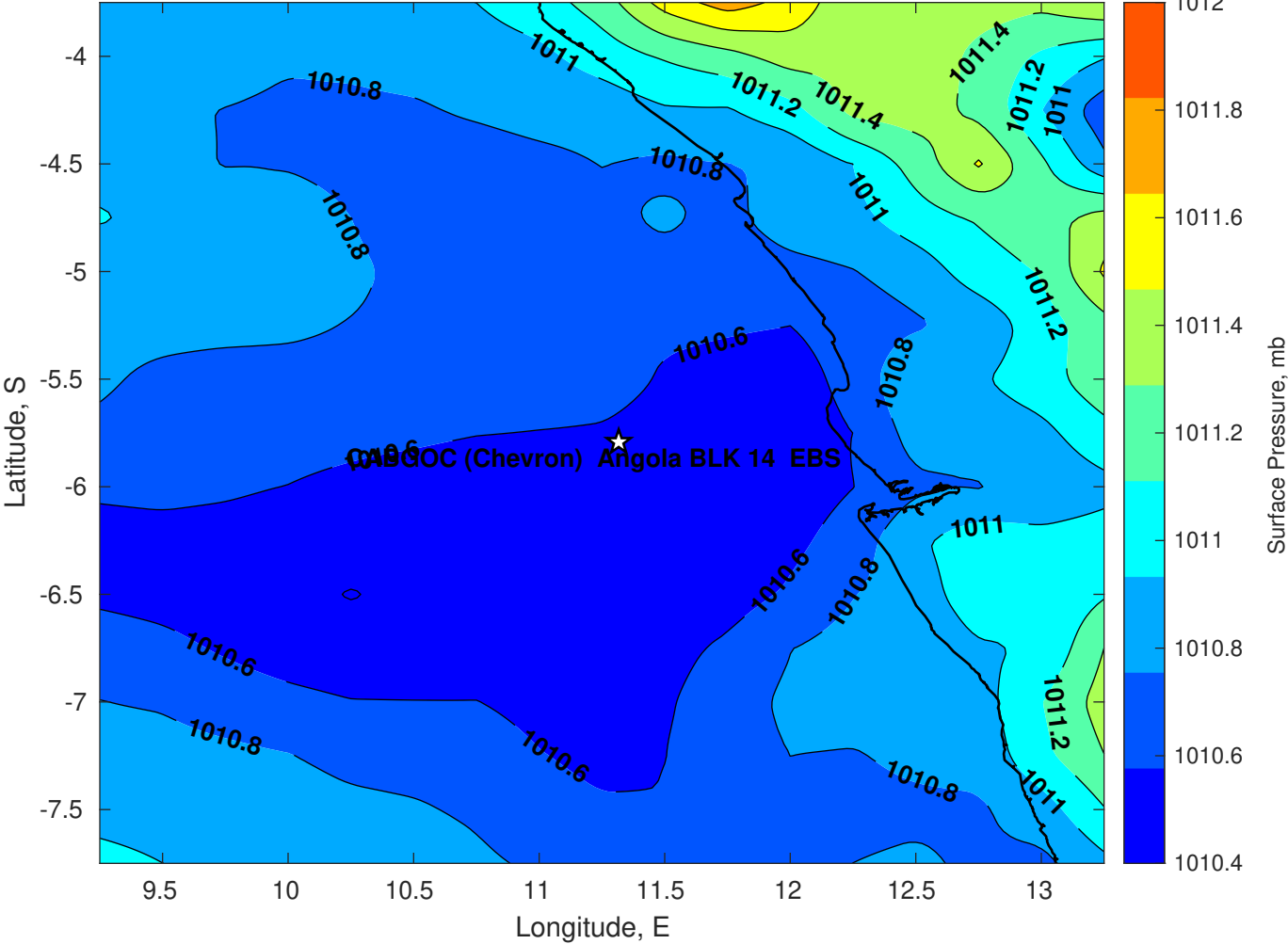
Surface Pressure (mb) for CABGOC (Chevron) Angola BLK 14 EBS at 15-Apr-2025 00:00:00
