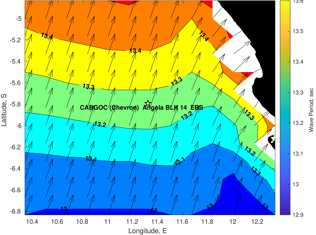
Wave Period (sec) for CABGOC (Chevron) Angola BLK 14 EBS at 15-Apr-2025 09:00:00
