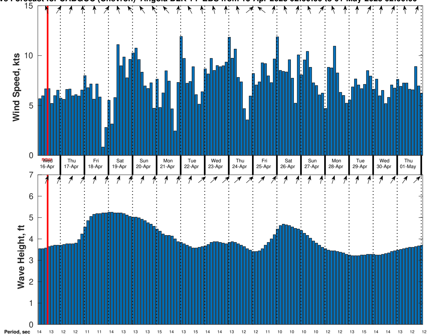
Wind & Wave Forecast for CABGOC (Chevron) Angola BLK 14 EBS from 15-Apr-2025 02:00:00 to 01-May-2025 02:00:00
