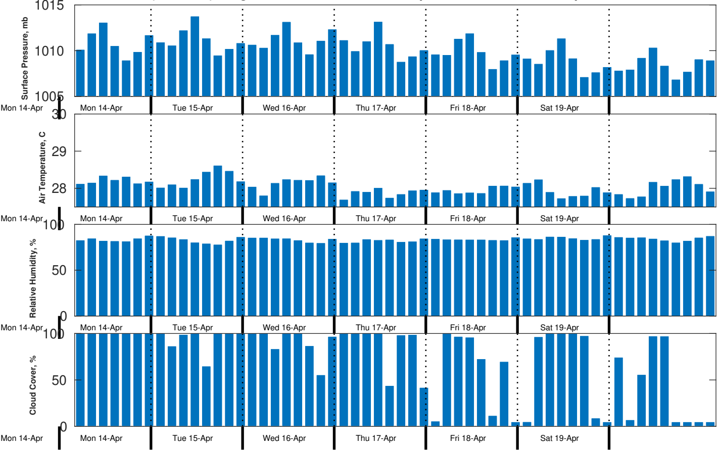
Met Forecast for CABGOC (Chevron) Angola BLK 14 EBS from 15-Apr-2025 00:00:00 to 22-Apr-2025 00:00:00
