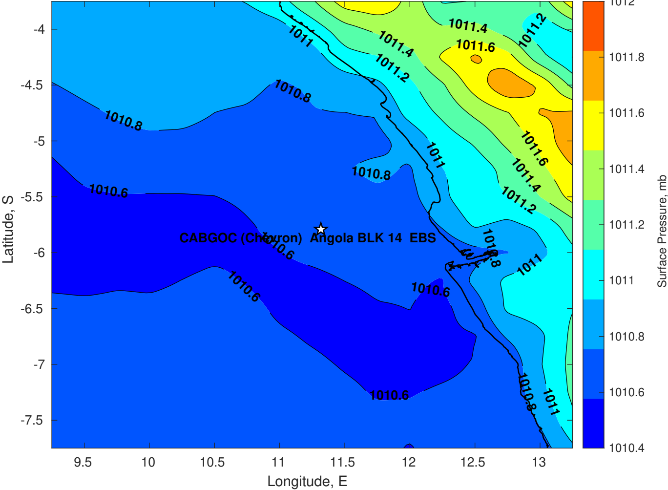
Surface Pressure (mb) for CABGOC (Chevron) Angola BLK 14 EBS at 17-Apr-2025 00:00:00
