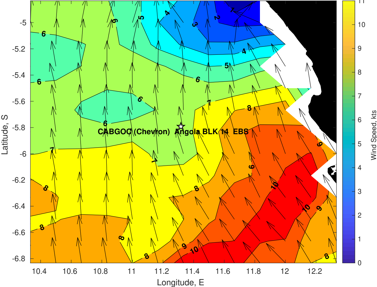
Winds (kts) for CABGOC (Chevron) Angola BLK 14 EBS at 15-Apr-2025 09:00:00
