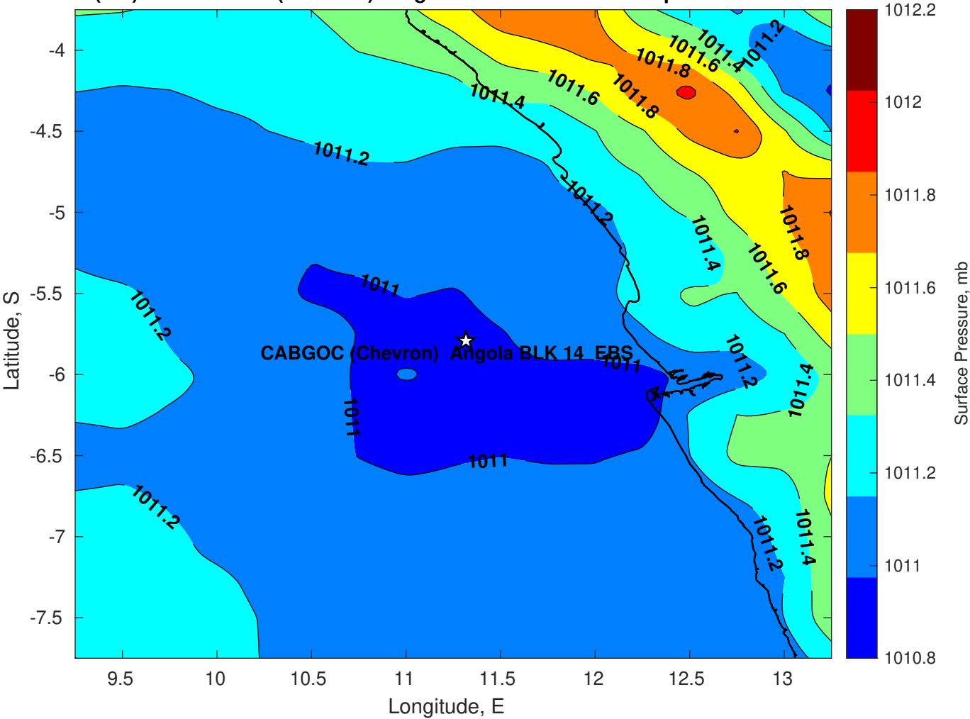
Surface Pressure (mb) for CABGOC (Chevron) Angola BLK 14 EBS at 16-Apr-2025 00:00:00
