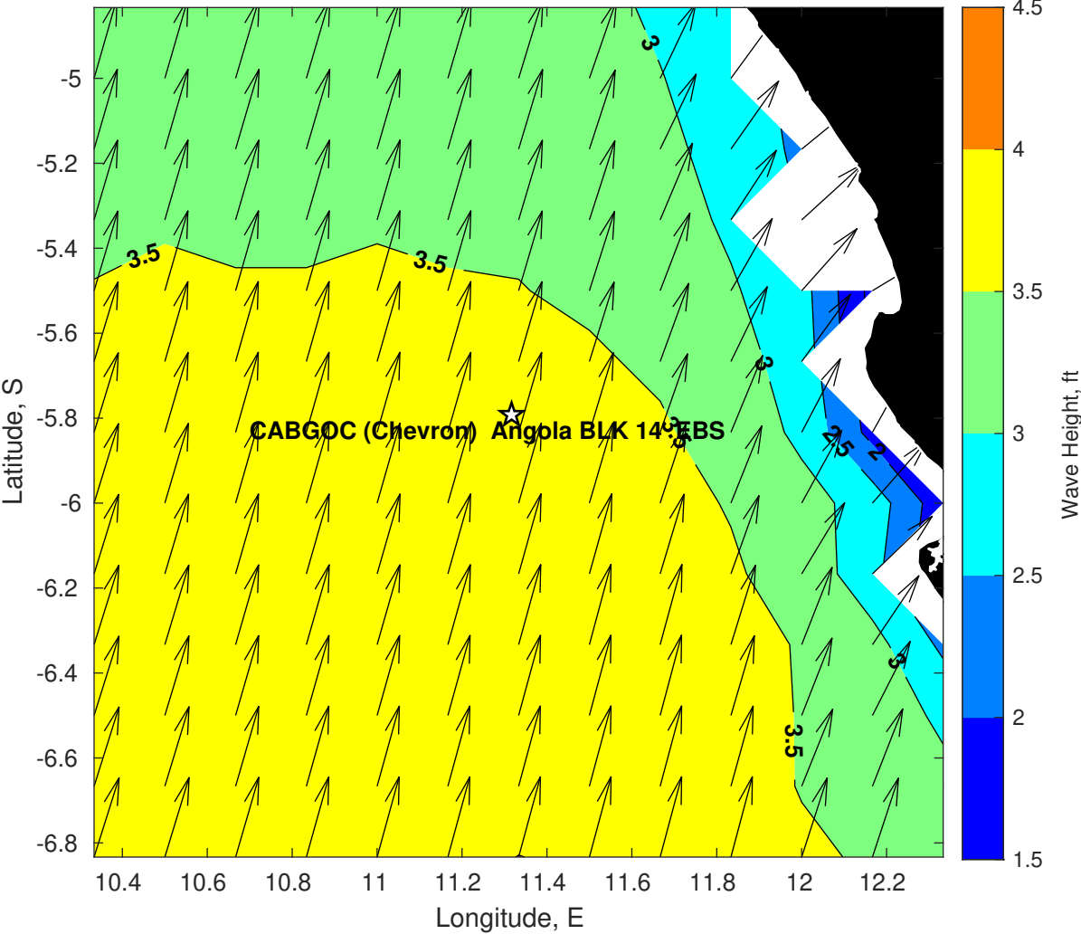
Wave Height (ft) for CABGOC (Chevron) Angola BLK 14 EBS at 15-Apr-2025 09:00:00
