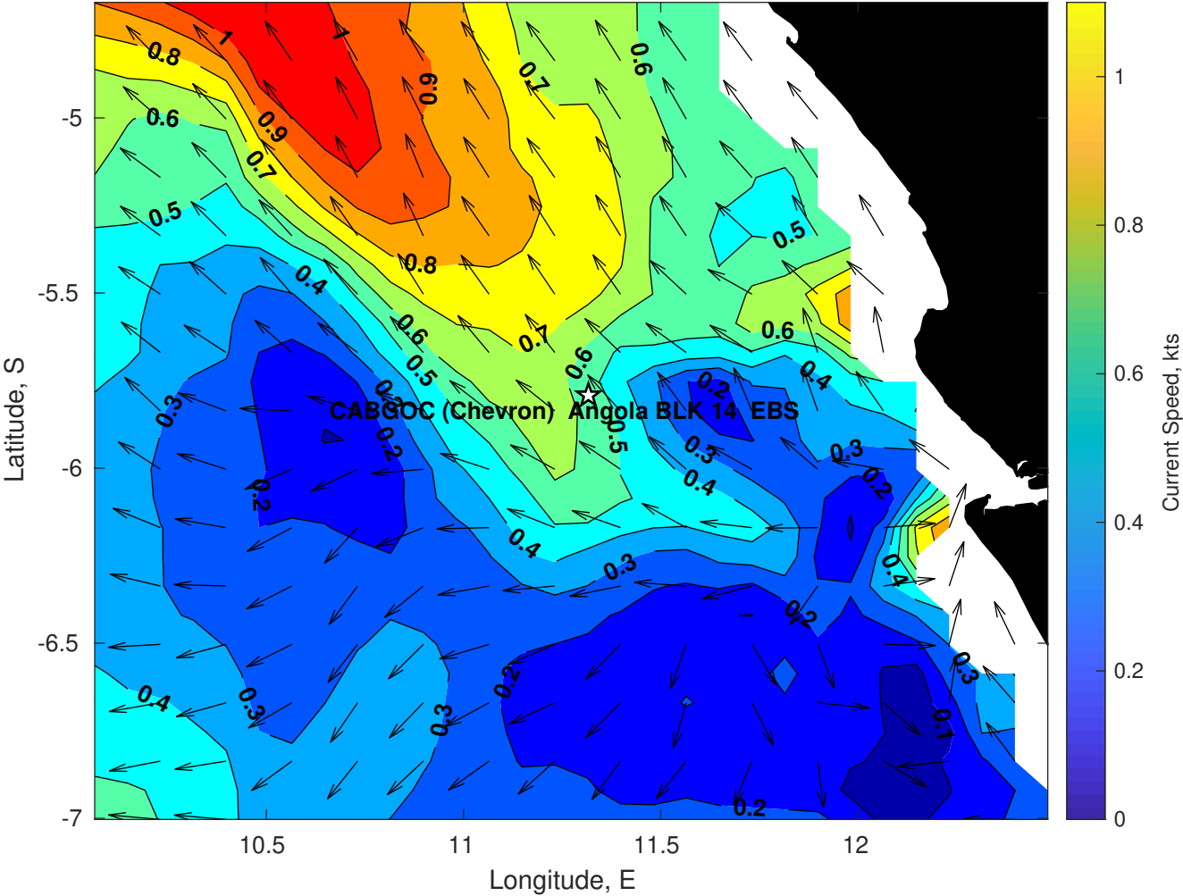
Surface Currents for CABGOC (Chevron) Angola BLK 14 EBS at 14-Apr-2025 00:00:00
