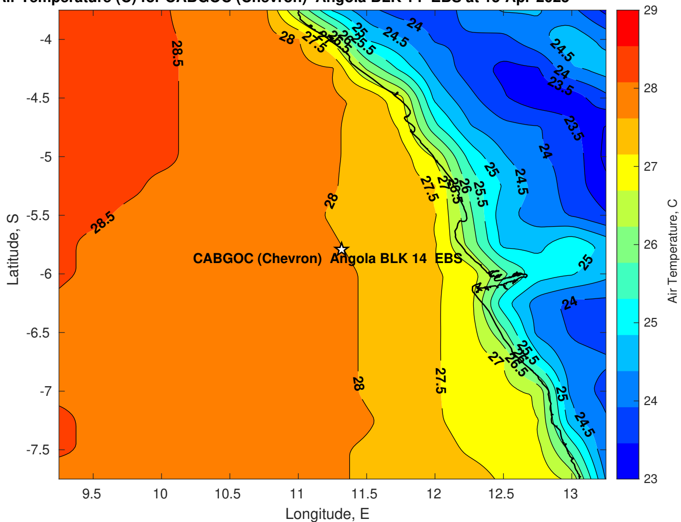
Air Temperature (C) for CABGOC (Chevron) Angola BLK 14 EBS at 15-Apr-2025
