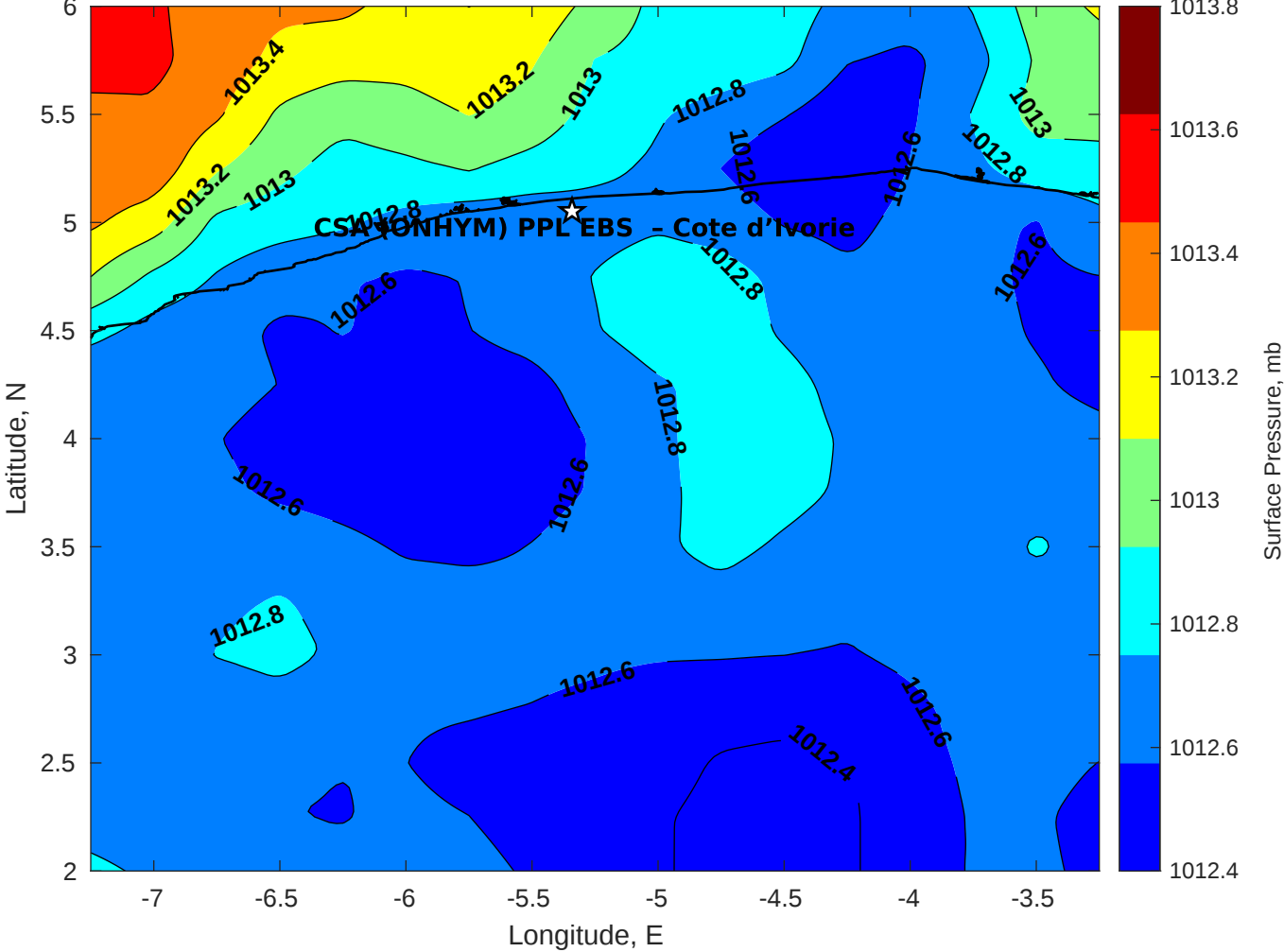
Surface Pressure (mb) for CSA (ONHYM) PPL EBS - Cote d'Ivoire at 16-Apr-2025 00:00:00
