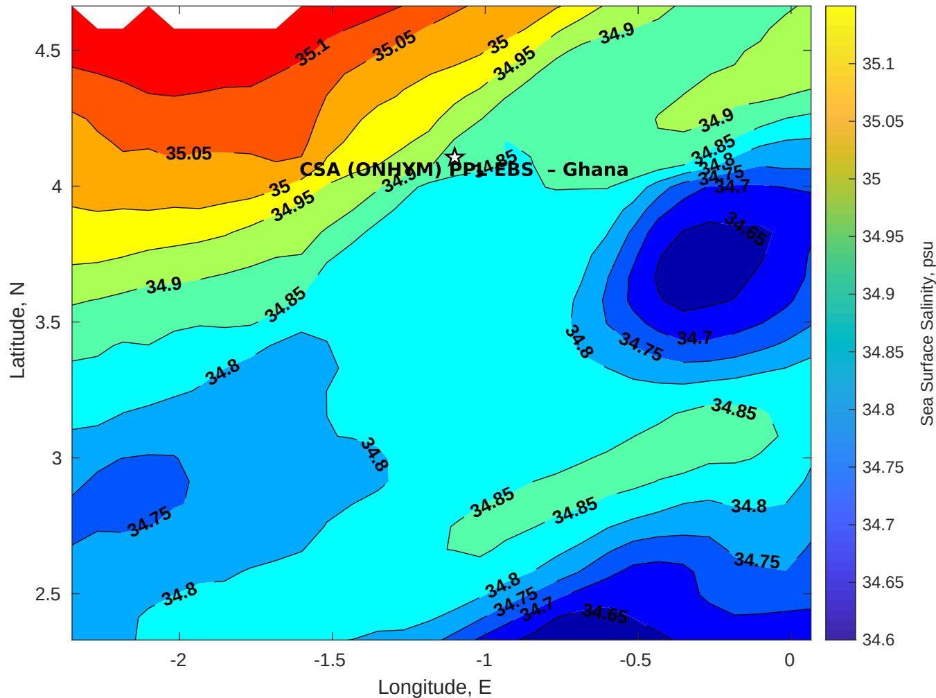
Surface Salinity for CSA (ONHYM) PPL EBS - Ghana at 14-Apr-2025 00:00:00
