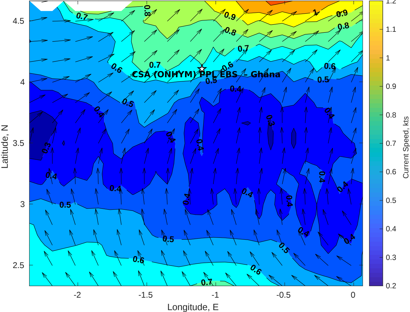
Surface Currents for CSA (ONHYM) PPL EBS - Ghana at 14-Apr-2025 00:00:00
