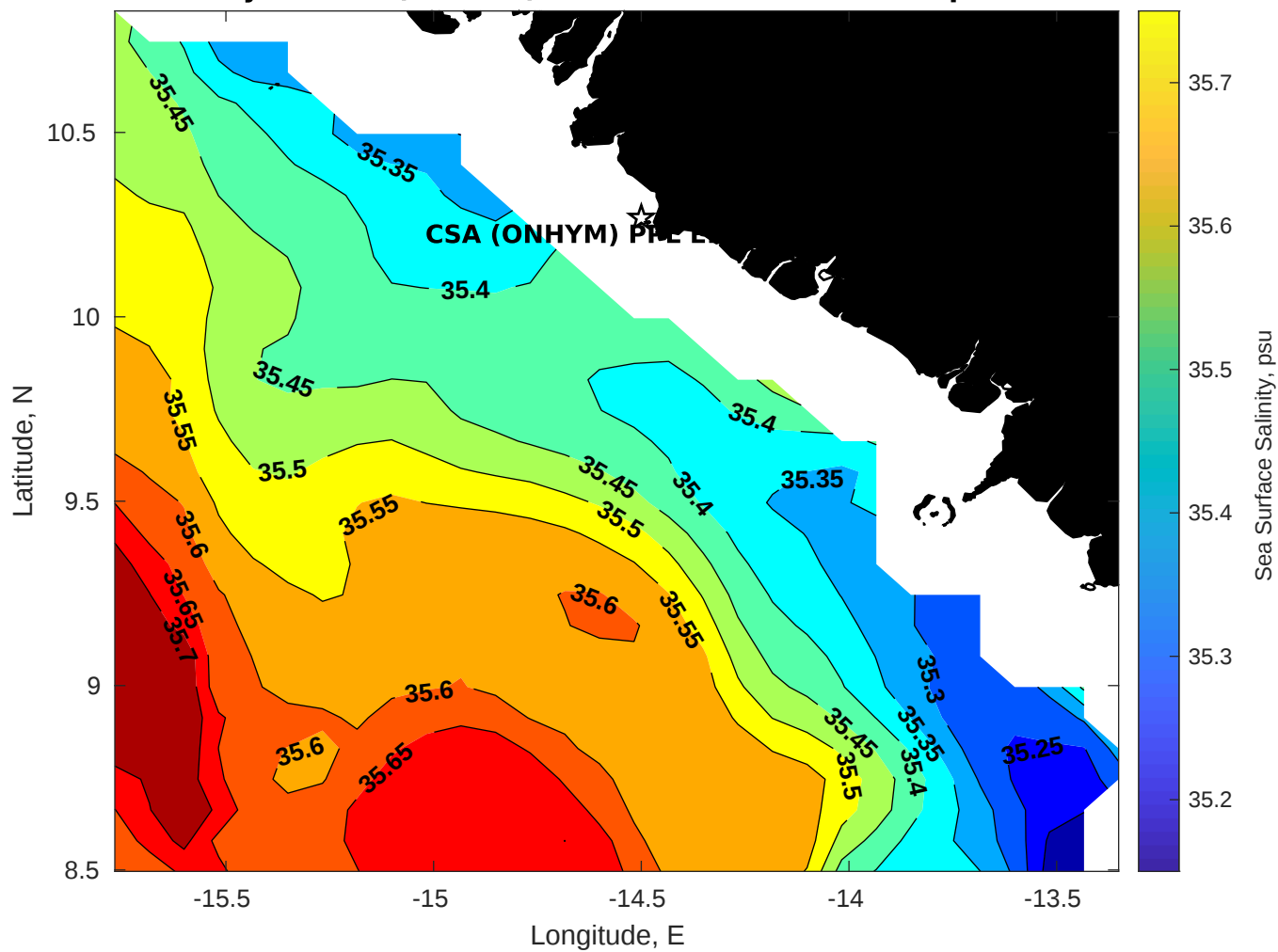
Surface Salinity for CSA (ONHYM) PPL EBS - Guinea at 14-Apr-2025 00:00:00
