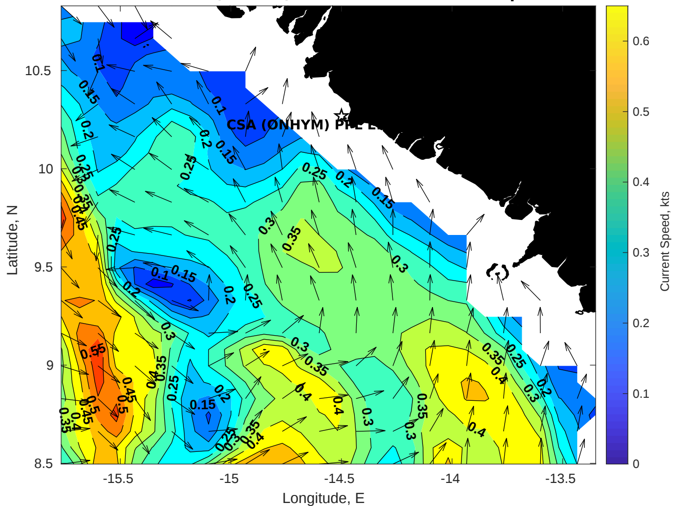
Surface Currents for CSA (ONHYM) PPL EBS - Guinea at 14-Apr-2025 00:00:00
