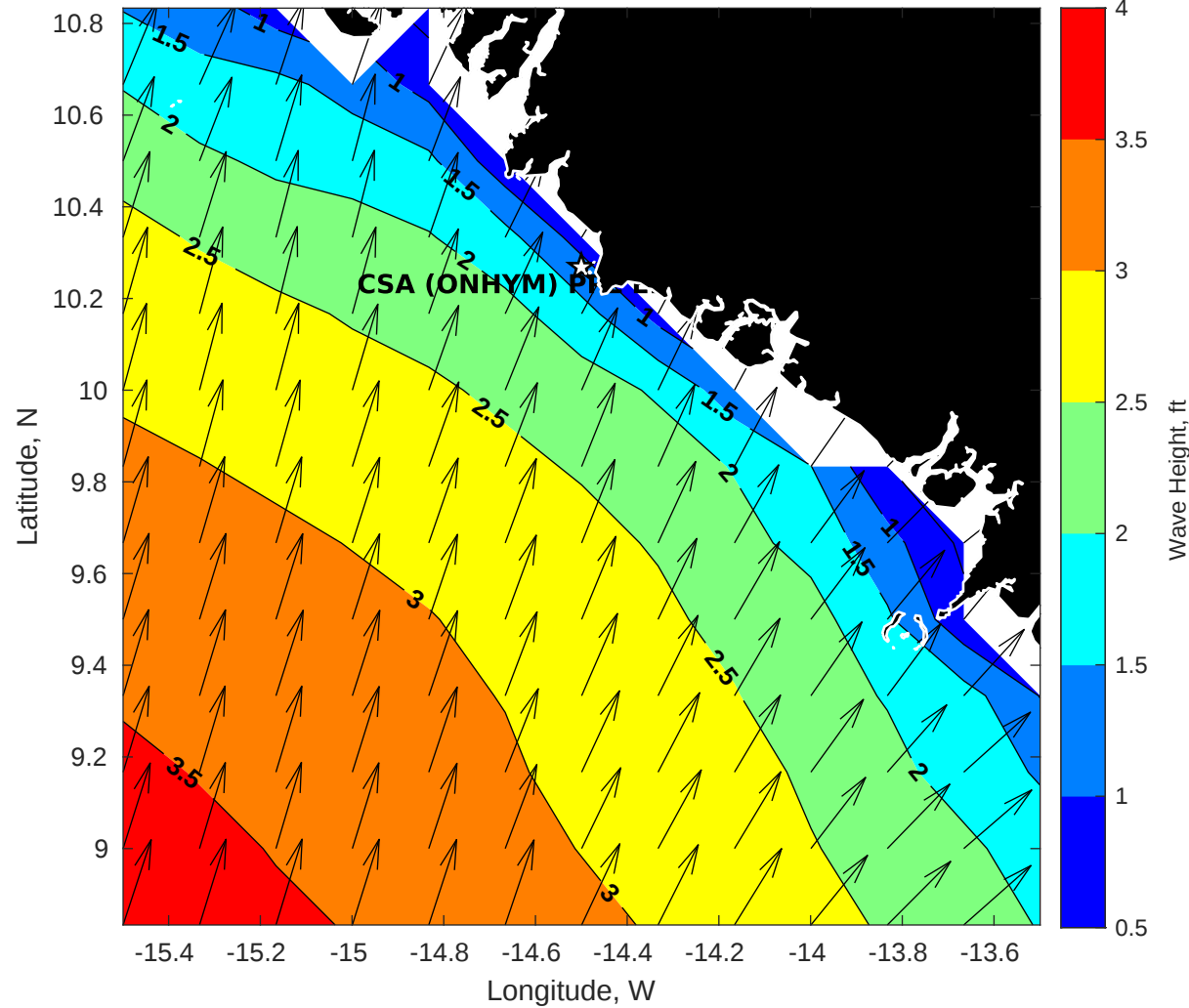
Wave Height (ft) for CSA (ONHYM) PPL EBS - Guinea at 15-Apr-2025 09:00:00
