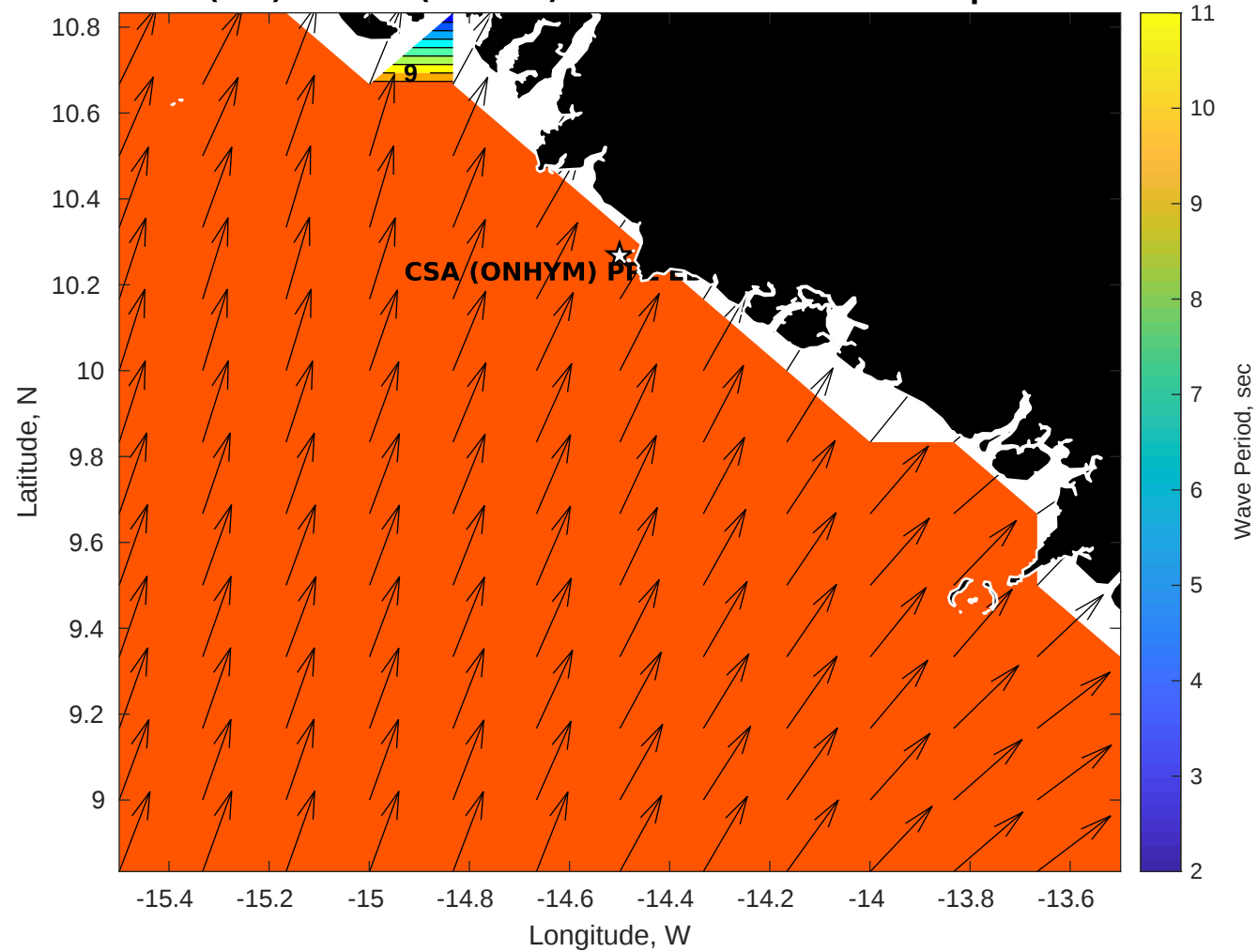
Wave Period (sec) for CSA (ONHYM) PPL EBS - Guinea at 15-Apr-2025 09:00:00
