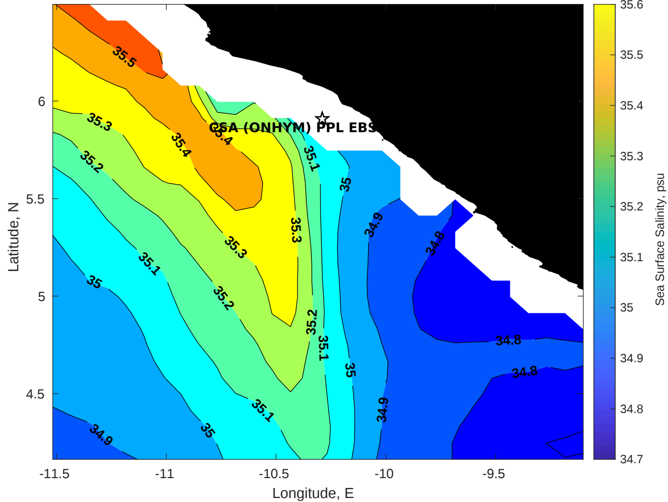
Surface Salinity for CSA (ONHYM) PPL EBS - Liberia at 14-Apr-2025 00:00:00
