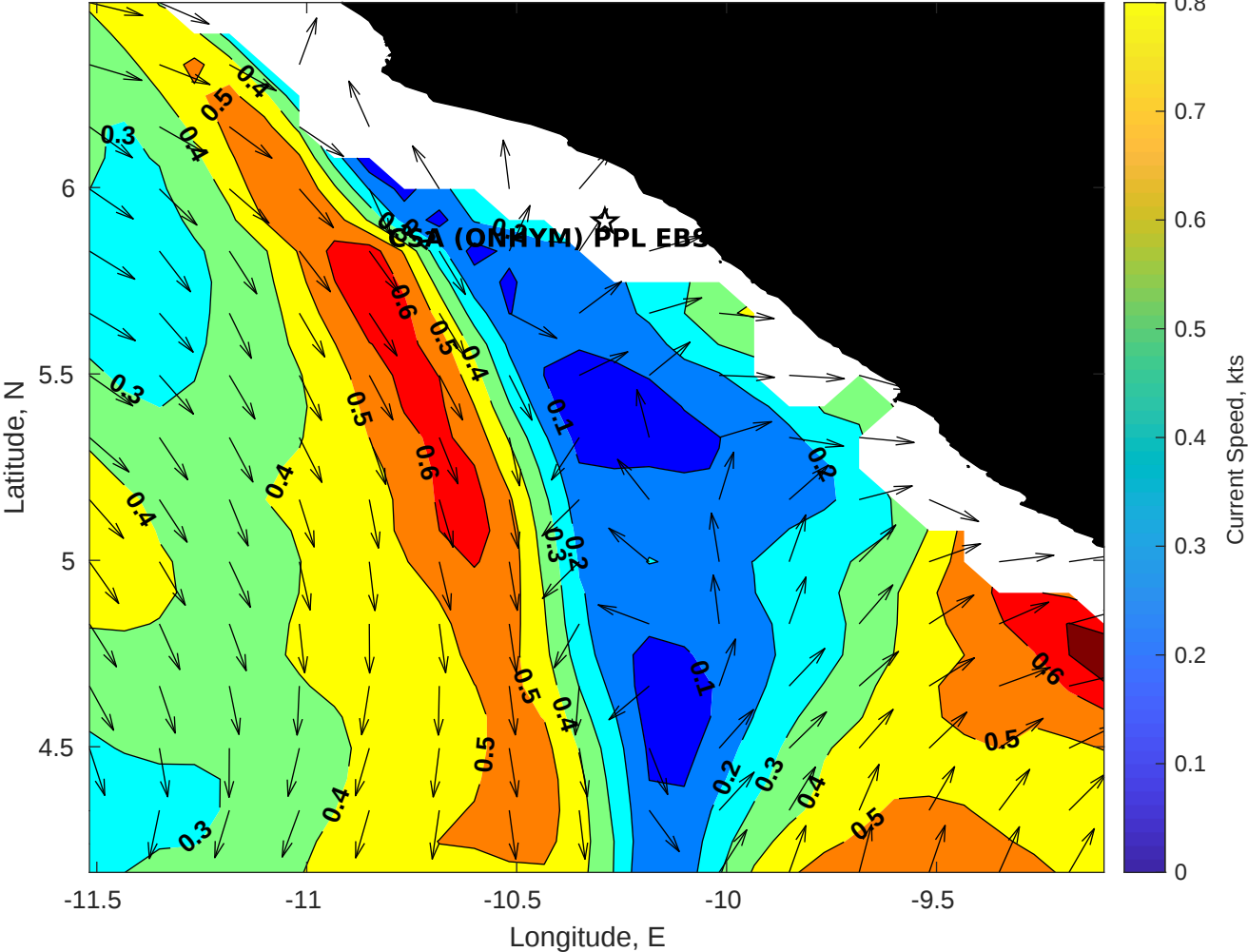
Surface Currents for CSA (ONHYM) PPL EBS - Liberia at 14-Apr-2025 00:00:00
