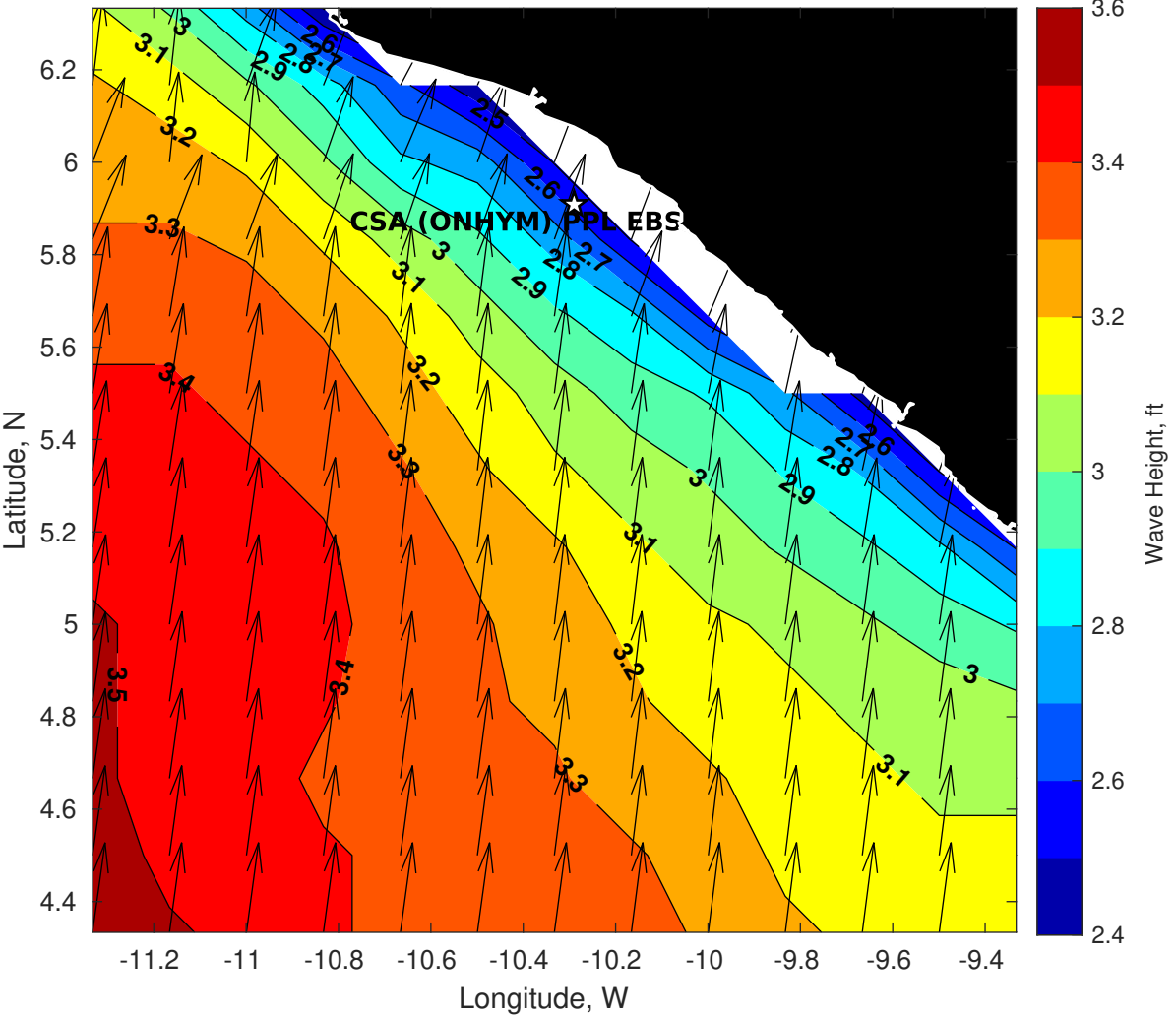
Wave Height (ft) for CSA (ONHYM) PPL EBS - Liberia at 15-Apr-2025 09:00:00
