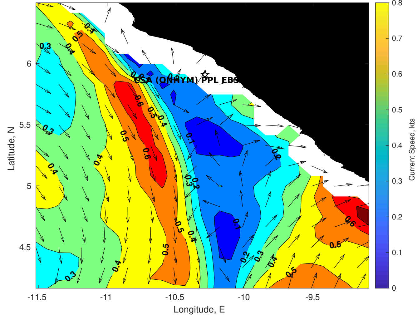
Surface Currents for CSA (ONHYM) PPL EBS - Liberia at 14-Apr-2025 00:00:00
