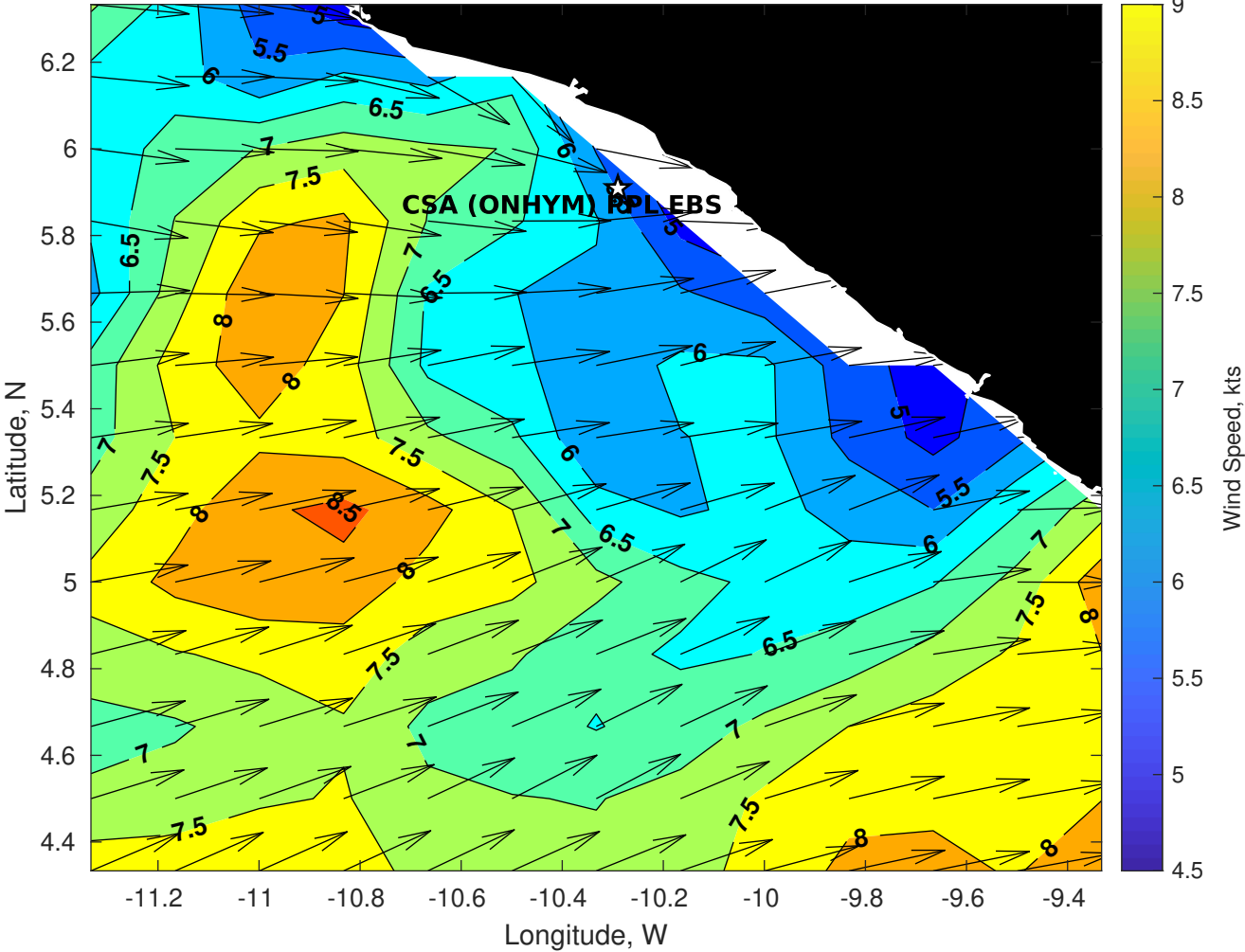
Winds (kts) for CSA (ONHYM) PPL EBS - Liberia at 15-Apr-2025 09:00:00
