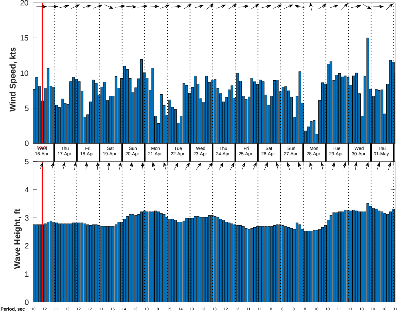
Wind & Wave Forecast for CSA (ONHYM) PPL EBS - Liberia from 15-Apr-2025 01:00:00 to 01-May-2025 01:00:00
