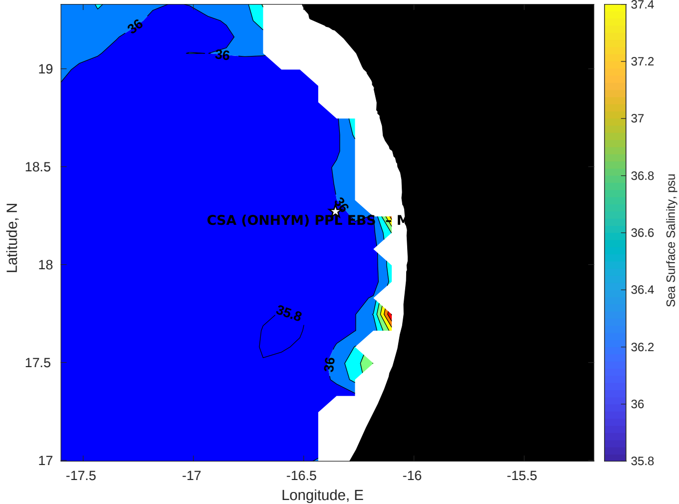
Surface Salinity for CSA (ONHYM) PPL EBS - Mauritania at 14-Apr-2025 00:00:00
