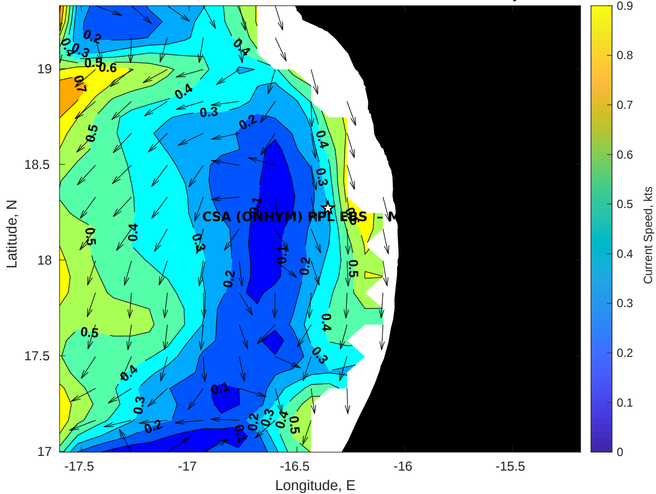
Surface Currents for CSA (ONHYM) PPL EBS - Mauritania at 14-Apr-2025 00:00:00
