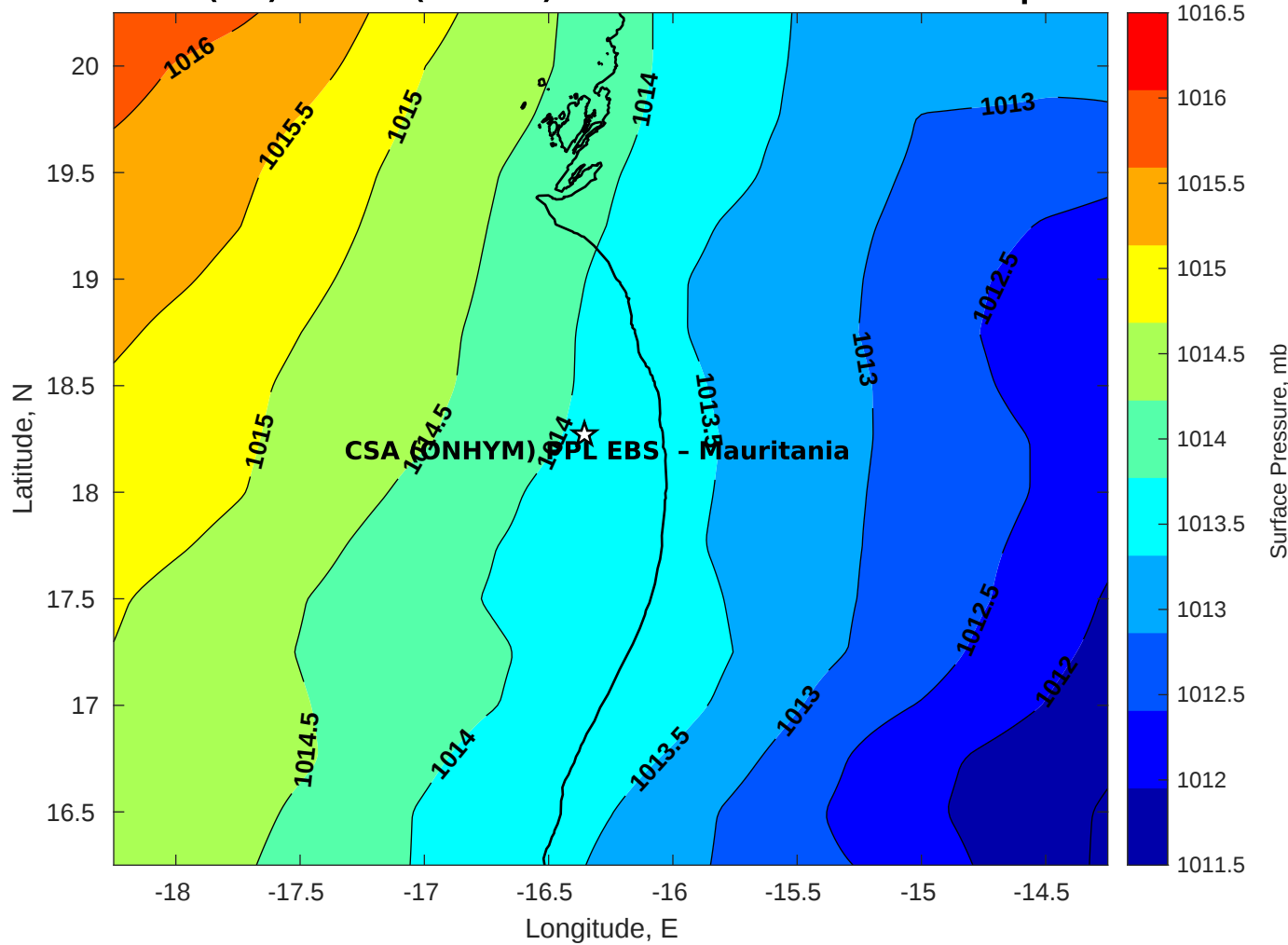
Surface Pressure (mb) for CSA (ONHYM) PPL EBS - Mauritania at 15-Apr-2025 00:00:00
