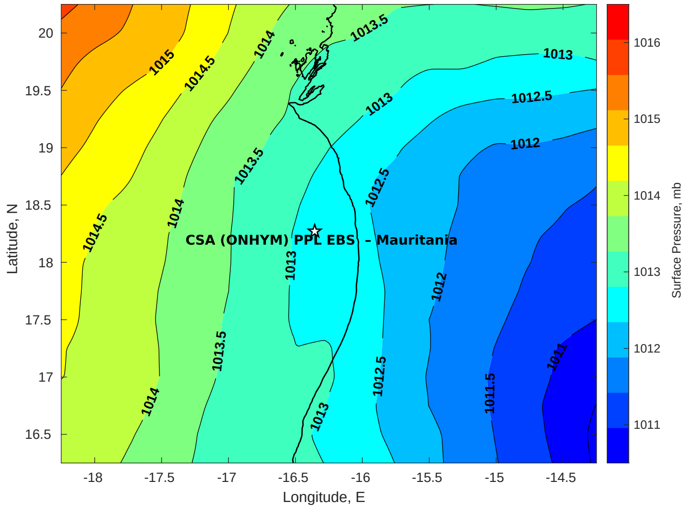
Surface Pressure (mb) for CSA (ONHYM) PPL EBS - Mauritania at 16-Apr-2025 00:00:00
