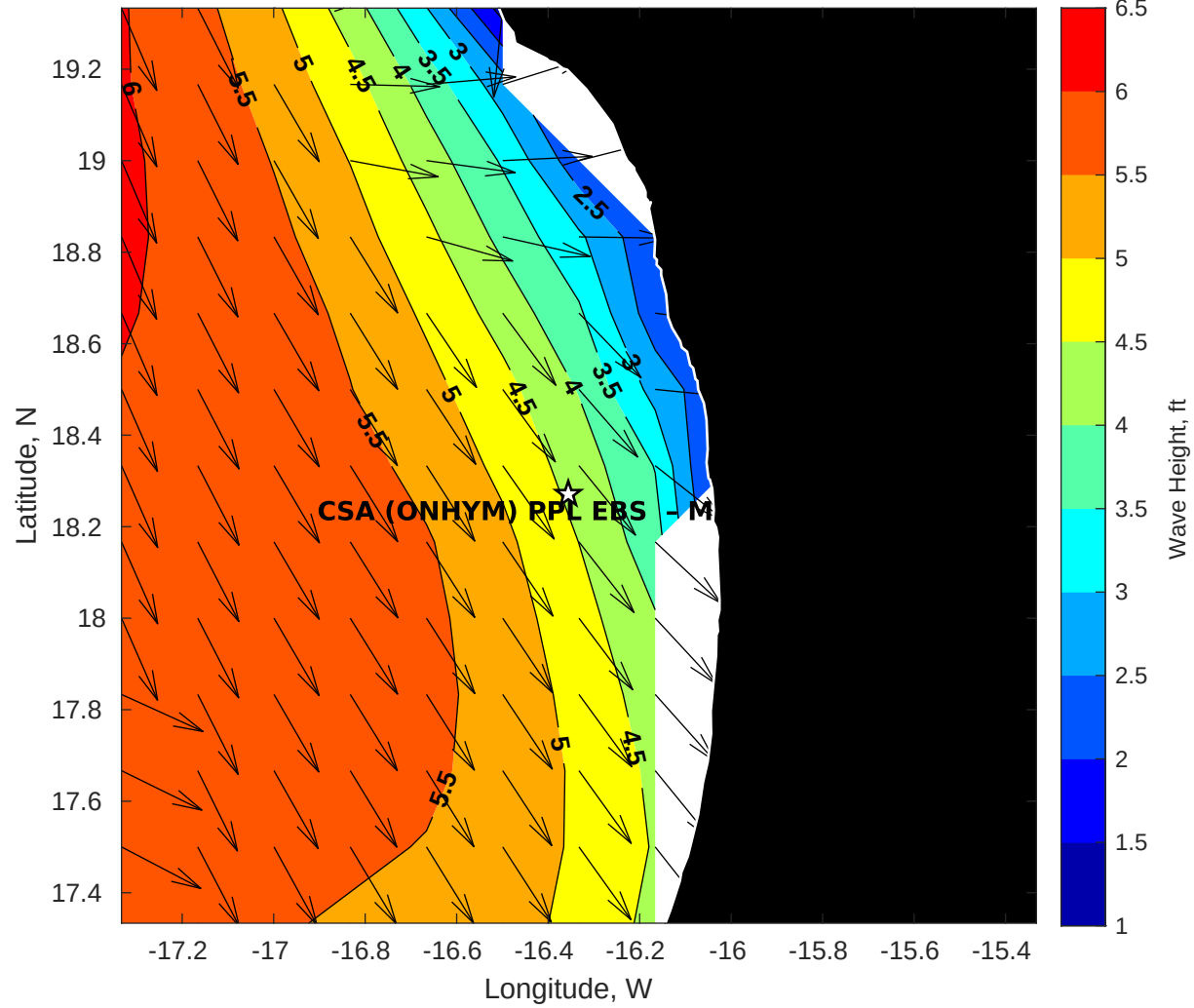
Wave Height (ft) for CSA (ONHYM) PPL EBS - Mauritania at 15-Apr-2025 09:00:00
