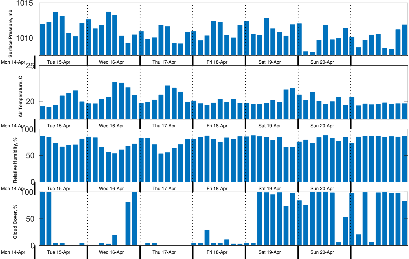
Met Forecast for CSA (ONHYM) PPL EBS - Mauritania from 15-Apr-2025 00:00:00 to 22-Apr-2025 00:00:00
