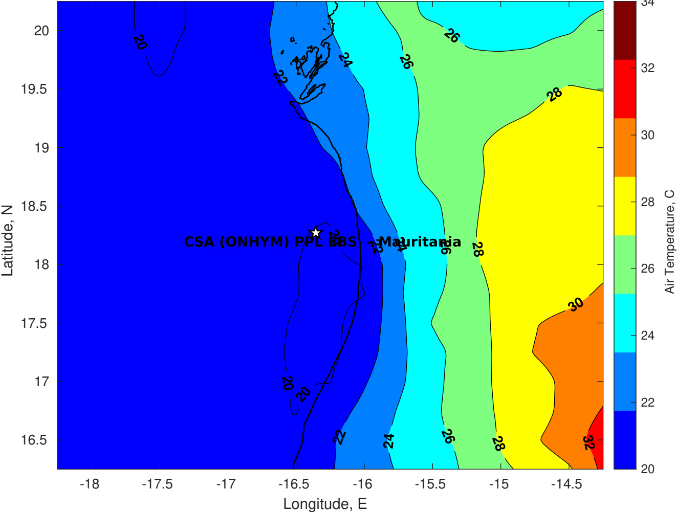
Air Temperature (C) for CSA (ONHYM) PPL EBS - Mauritania at 15-Apr-2025
