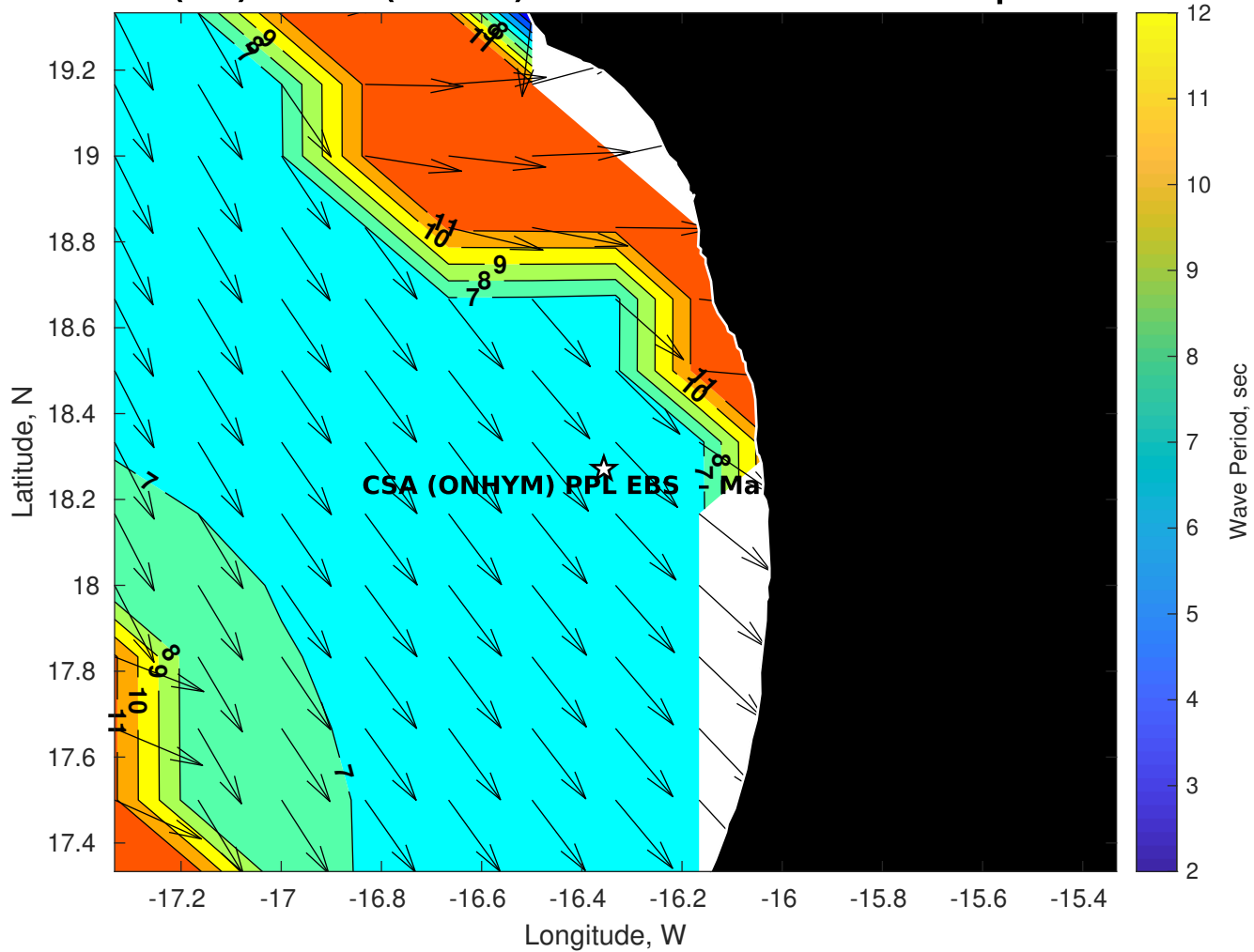
Wave Period (sec) for CSA (ONHYM) PPL EBS - Mauritania at 15-Apr-2025 09:00:00
