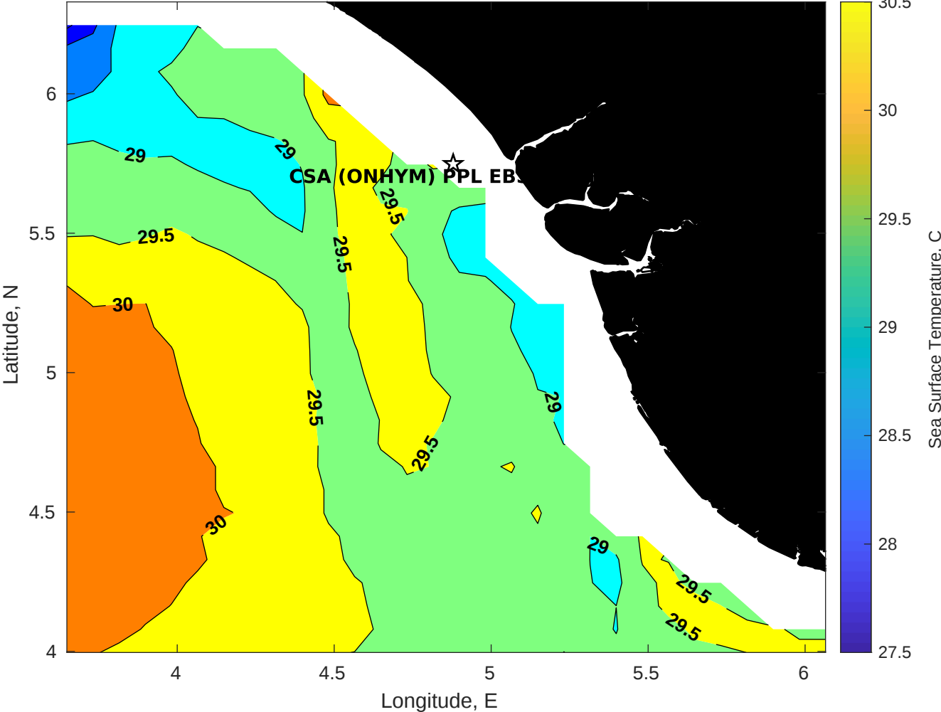
SST for CSA (ONHYM) PPL EBS - Nigeria at 14-Apr-2025 00:00:00
