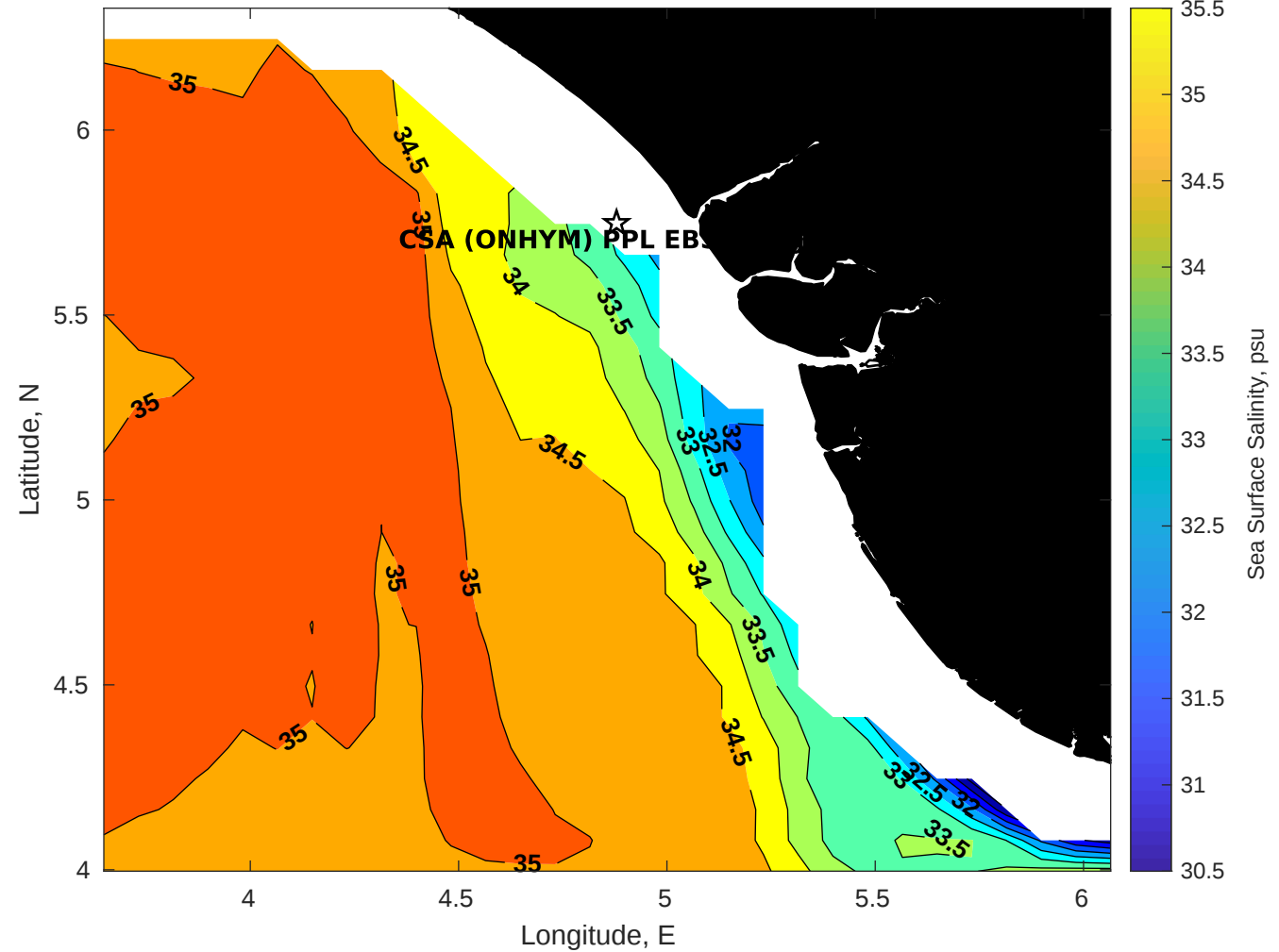
Surface Salinity for CSA (ONHYM) PPL EBS - Nigeria at 14-Apr-2025 00:00:00
