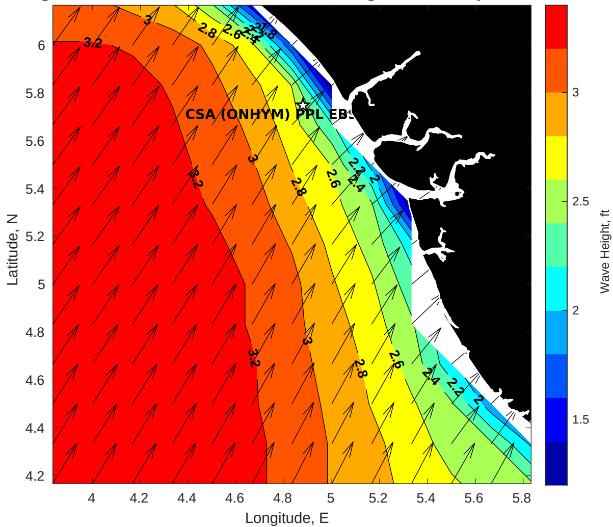
Wave Height (ft) for CSA (ONHYM) PPL EBS - Nigeria at 15-Apr-2025 09:00:00
