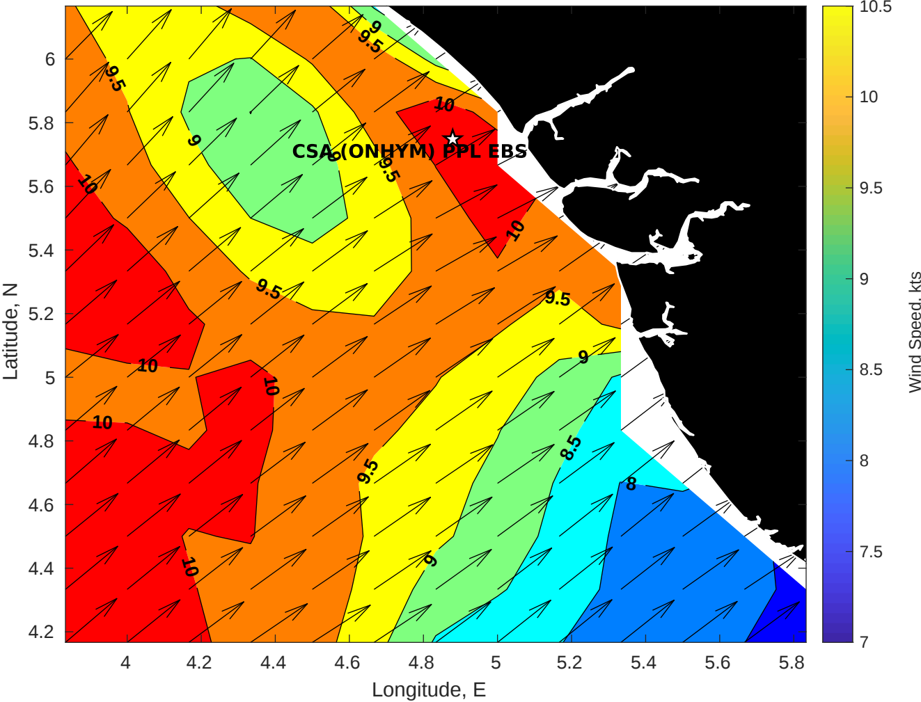
Winds (kts) for CSA (ONHYM) PPL EBS - Nigeria at 15-Apr-2025 09:00:00
