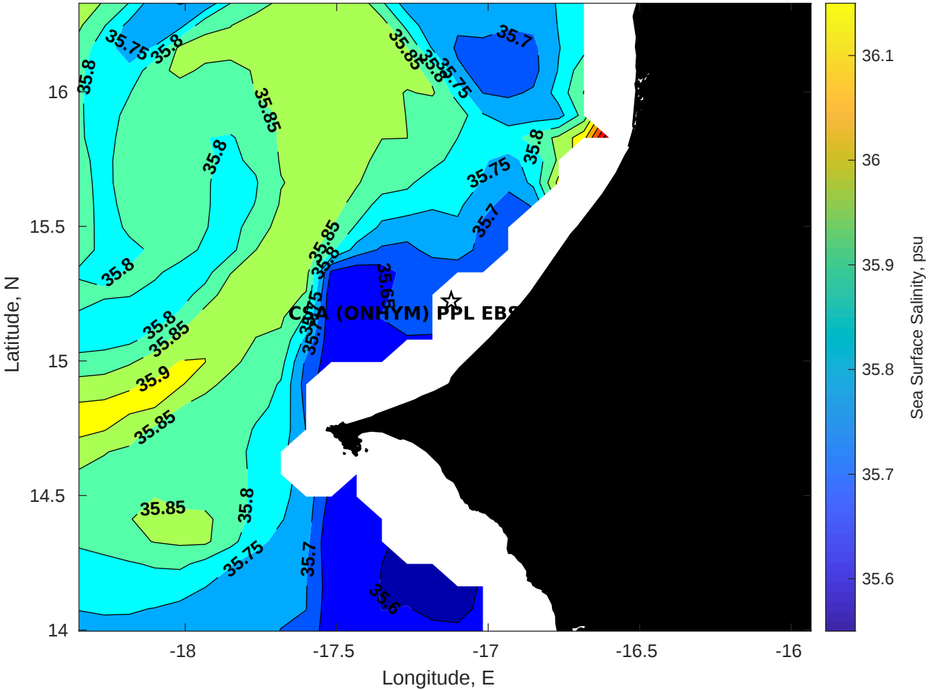
Surface Salinity for CSA (ONHYM) PPL EBS - Senegal at 14-Apr-2025 00:00:00
