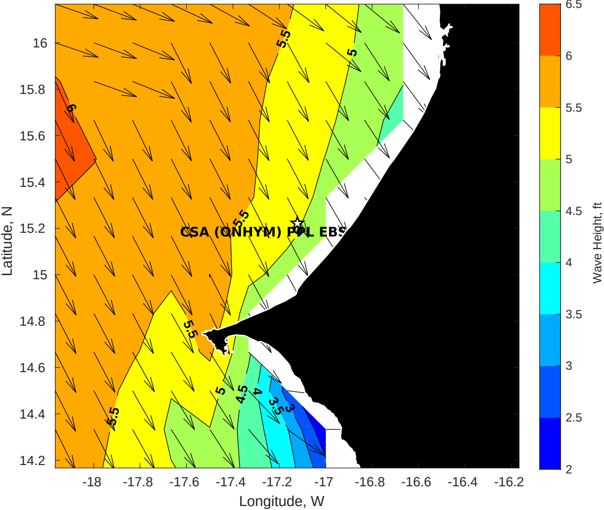
Wave Height (ft) for CSA (ONHYM) PPL EBS - Senegal at 15-Apr-2025 09:00:00
