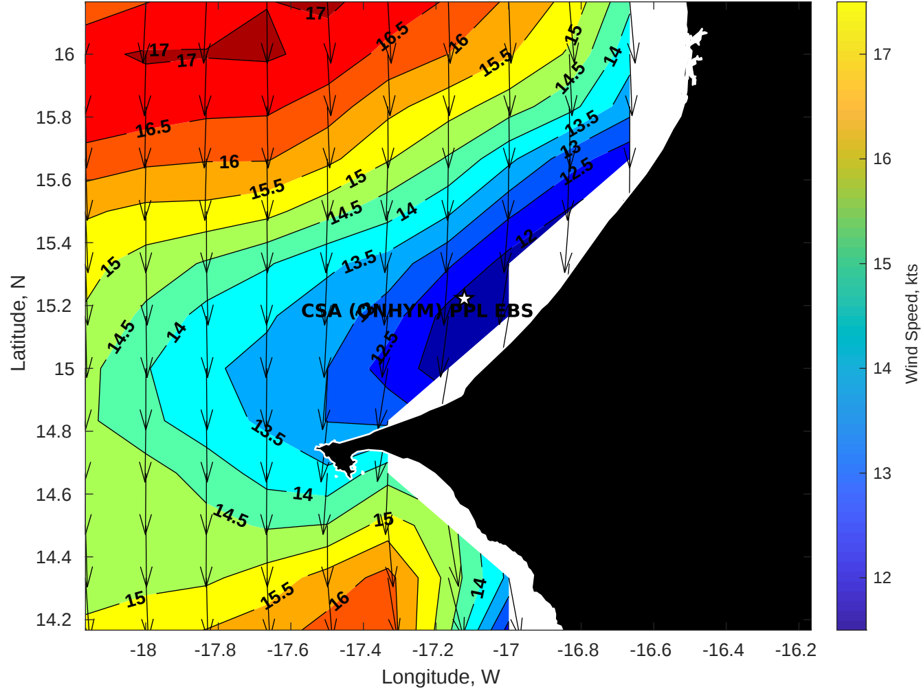
Winds (kts) for CSA (ONHYM) PPL EBS - Senegal at 15-Apr-2025 09:00:00
