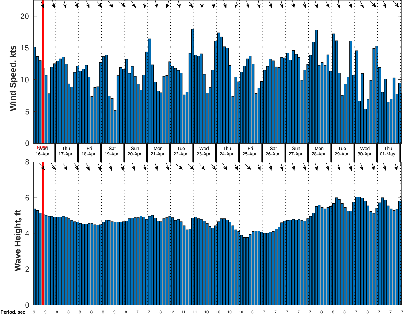
Wind & Wave Forecast for CSA (ONHYM) PPL EBS - Senegal from 15-Apr-2025 01:00:00 to 01-May-2025 01:00:00
