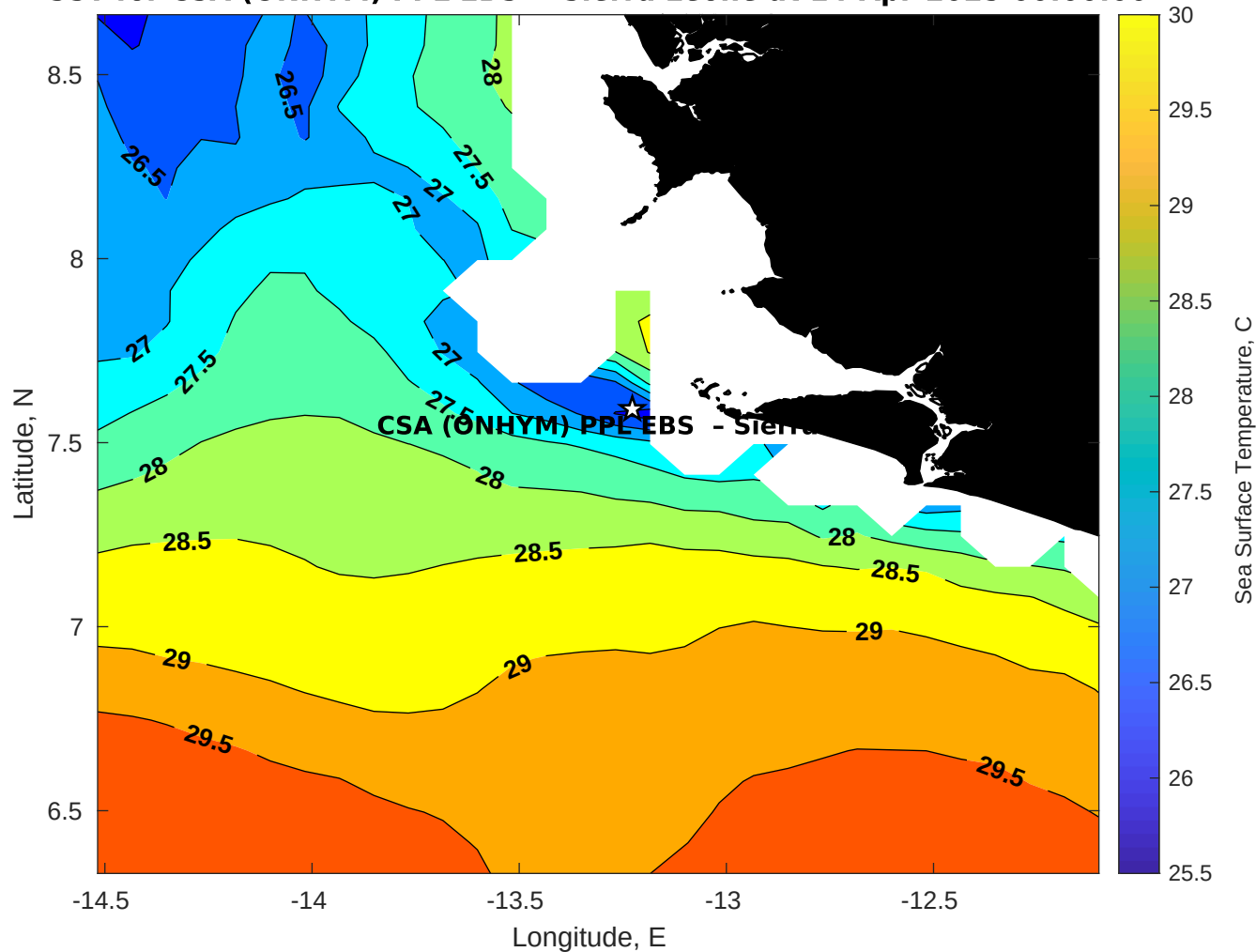
SST for CSA (ONHYM) PPL EBS - Sierra Leone at 14-Apr-2025 00:00:00
