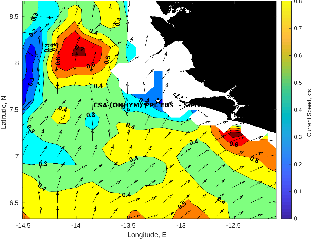
Surface Currents for CSA (ONHYM) PPL EBS - Sierra Leone at 14-Apr-2025 00:00:00
