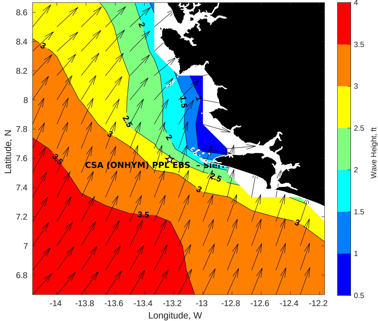
Wave Height (ft) for CSA (ONHYM) PPL EBS - Sierra Leone at 15-Apr-2025 09:00:00
