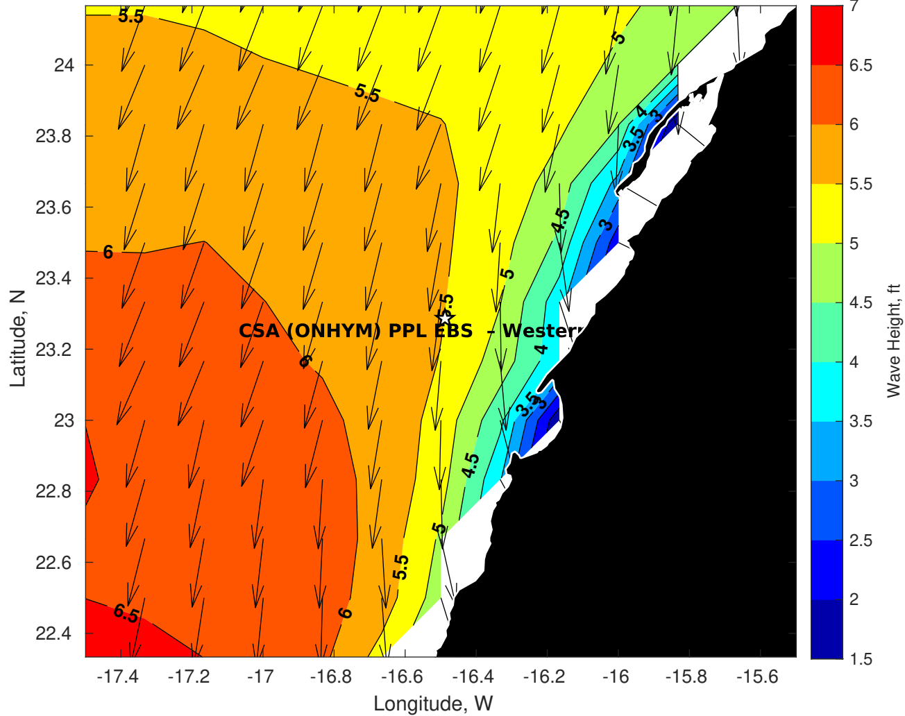
Wave Height (ft) for CSA (ONHYM) PPL EBS - Western Sahara at 15-Apr-2025 09:00:00
