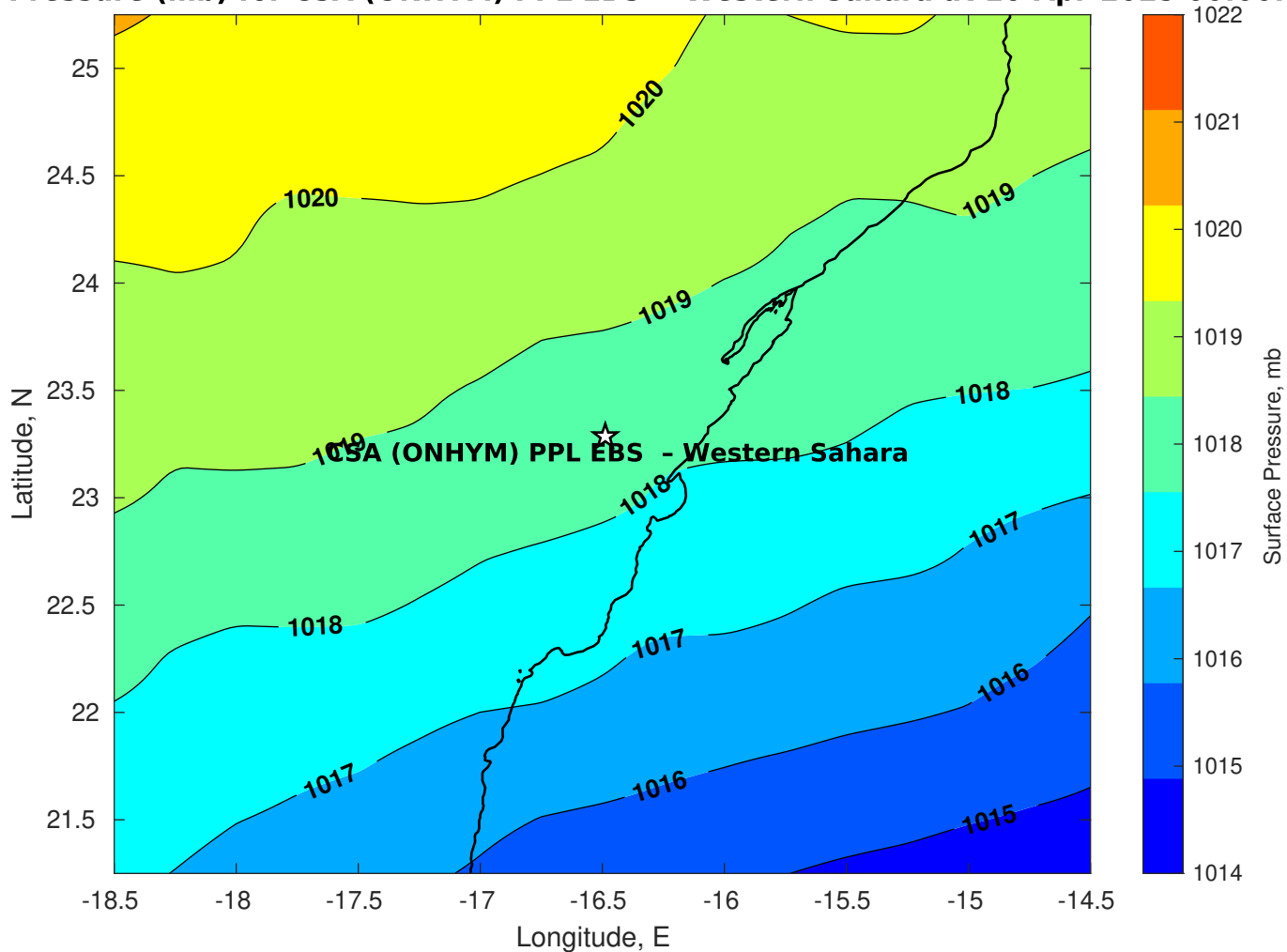
Surface Pressure (mb) for CSA (ONHYM) PPL EBS - Western Sahara at 16-Apr-2025 00:00:00
