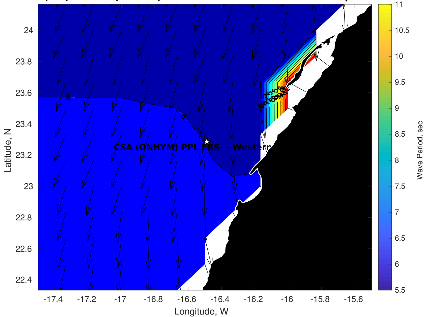
Wave Period (sec) for CSA (ONHYM) PPL EBS - Western Sahara at 15-Apr-2025 09:00:00
