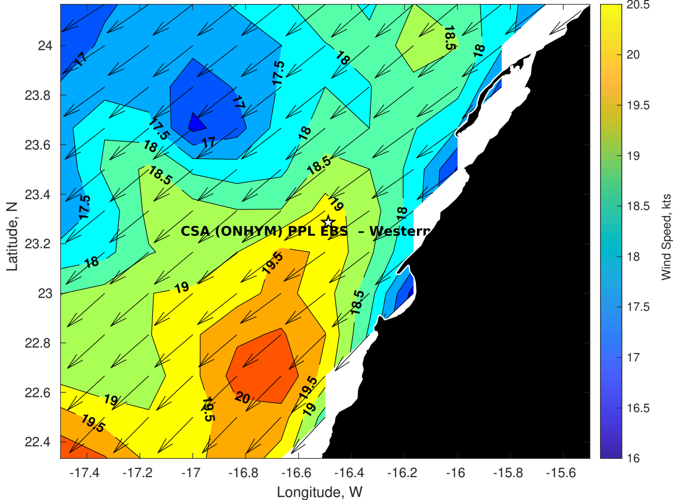
Winds (kts) for CSA (ONHYM) PPL EBS - Western Sahara at 15-Apr-2025 09:00:00
