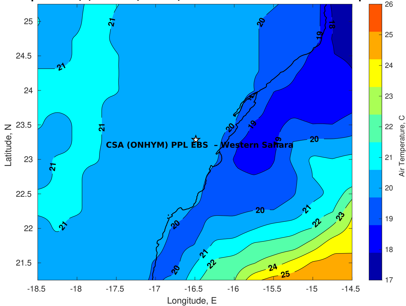
Air Temperature (C) for CSA (ONHYM) PPL EBS - Western Sahara at 15-Apr-2025
