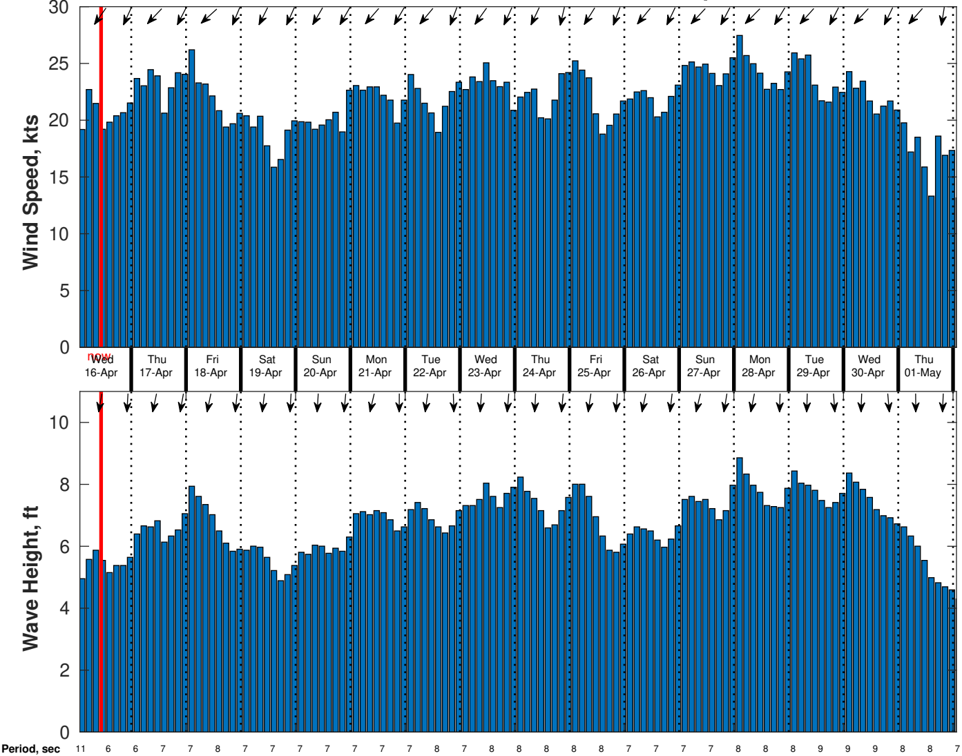
Wind & Wave Forecast for CSA (ONHYM) PPL EBS - Western Sahara from 15-Apr-2025 01:00:00 to 01-May-2025 01:00:00
