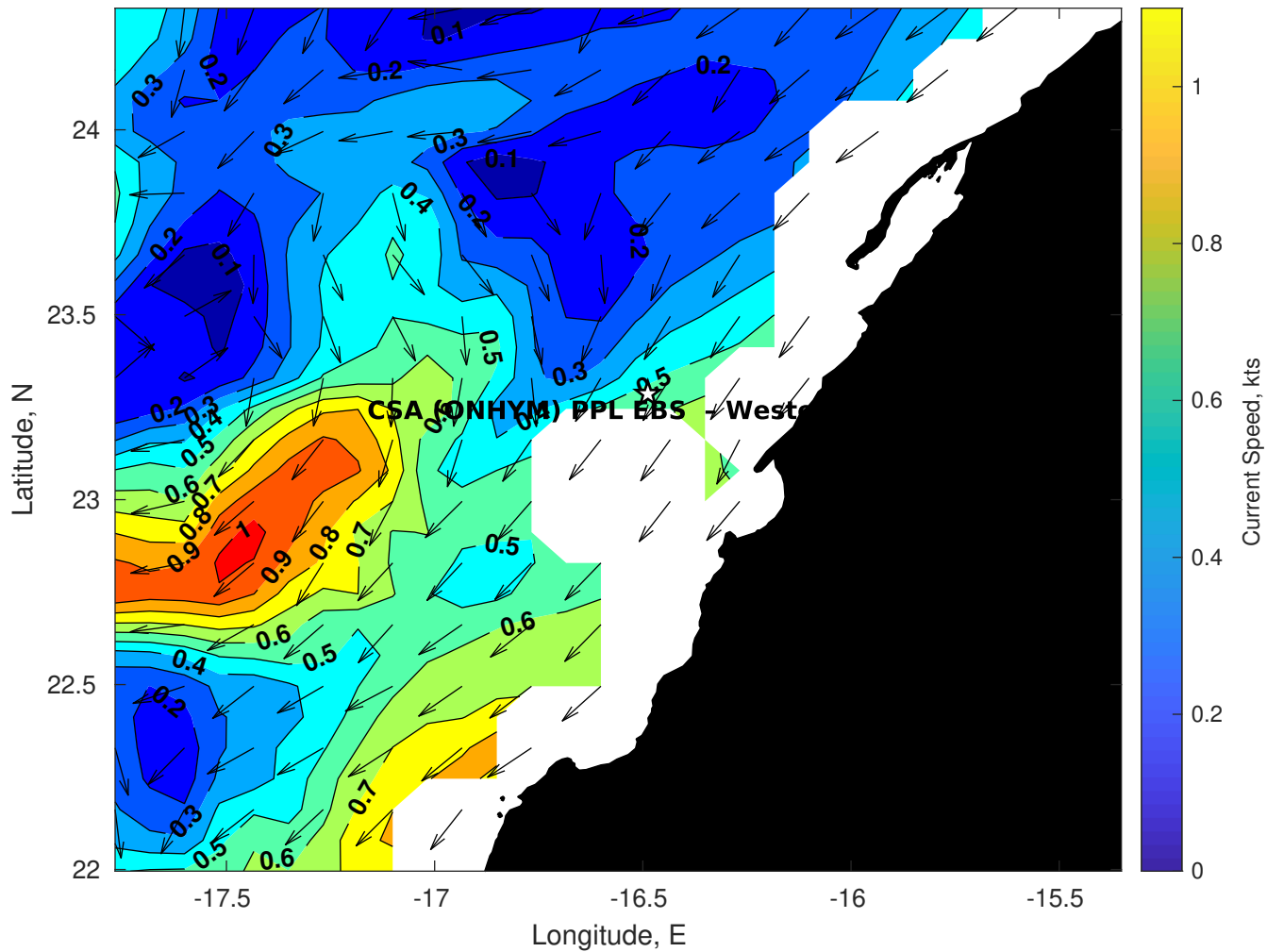
Surface Currents for CSA (ONHYM) PPL EBS - Western Sahara at 14-Apr-2025 00:00:00
