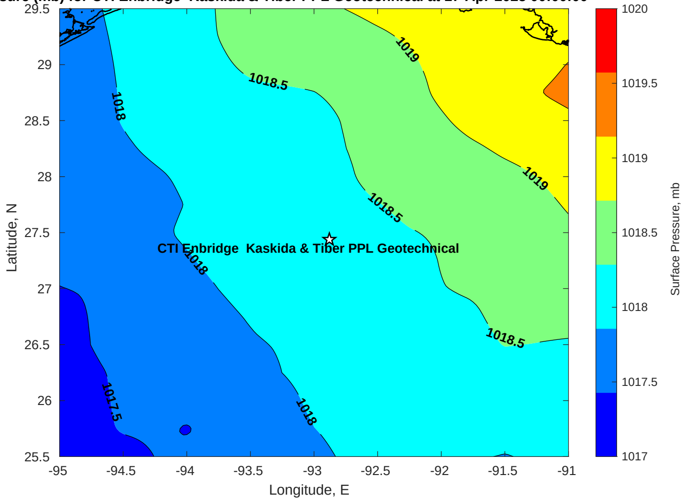
Surface Pressure (mb) for CTI Enbridge Kaskida & Tiber PPL Geotechnical at 17-Apr-2025 00:00:00
