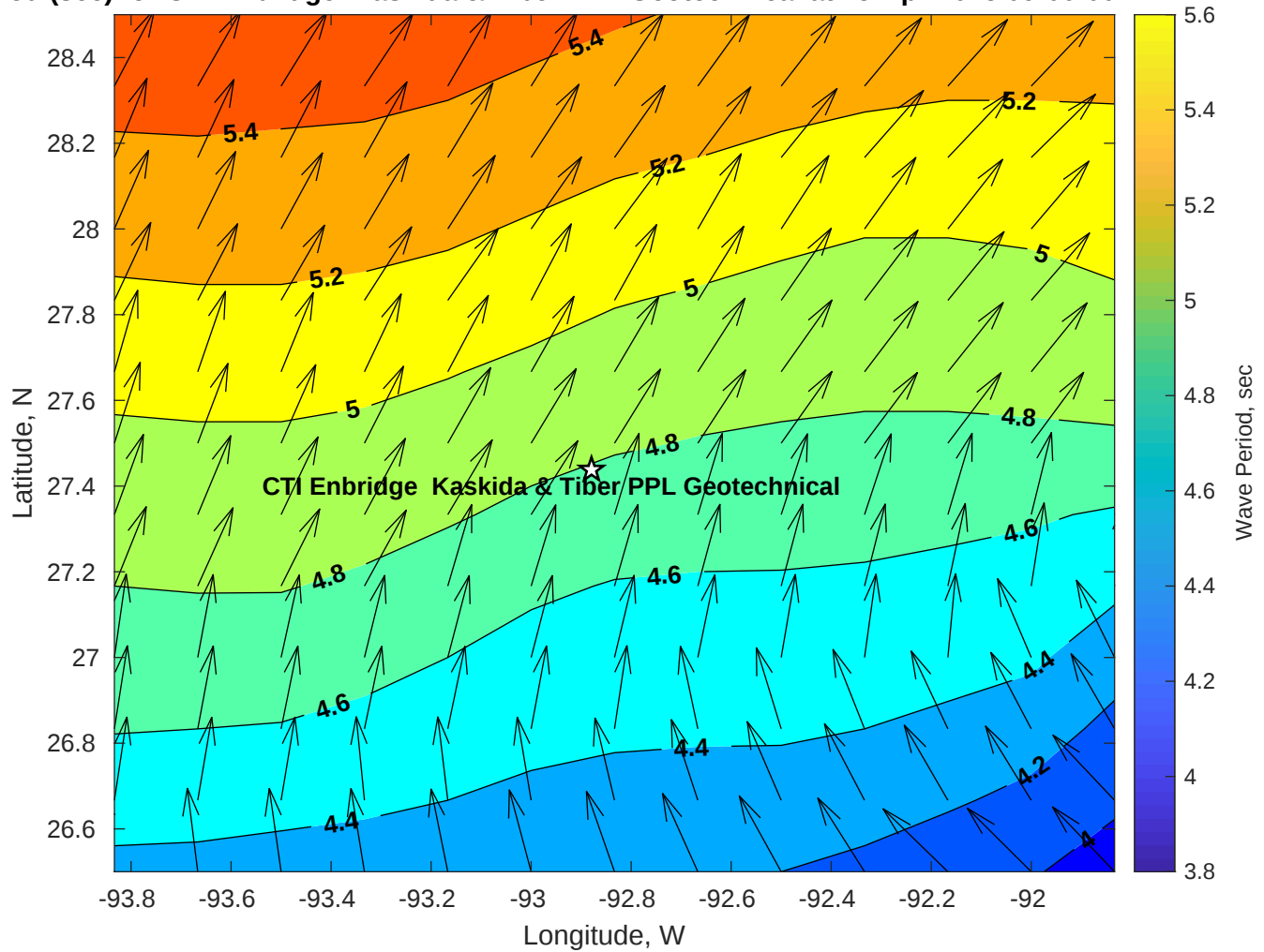
Wave Period (sec) for CTI Enbridge Kaskida & Tiber PPL Geotechnical at 15-Apr-2025 09:00:00
