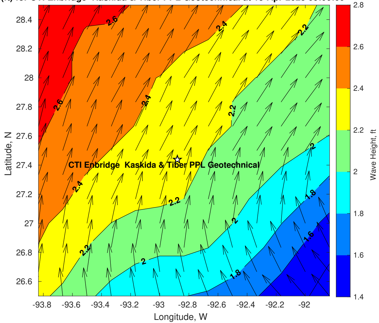
Wave Height (ft) for CTI Enbridge Kaskida & Tiber PPL Geotechnical at 15-Apr-2025 09:00:00
