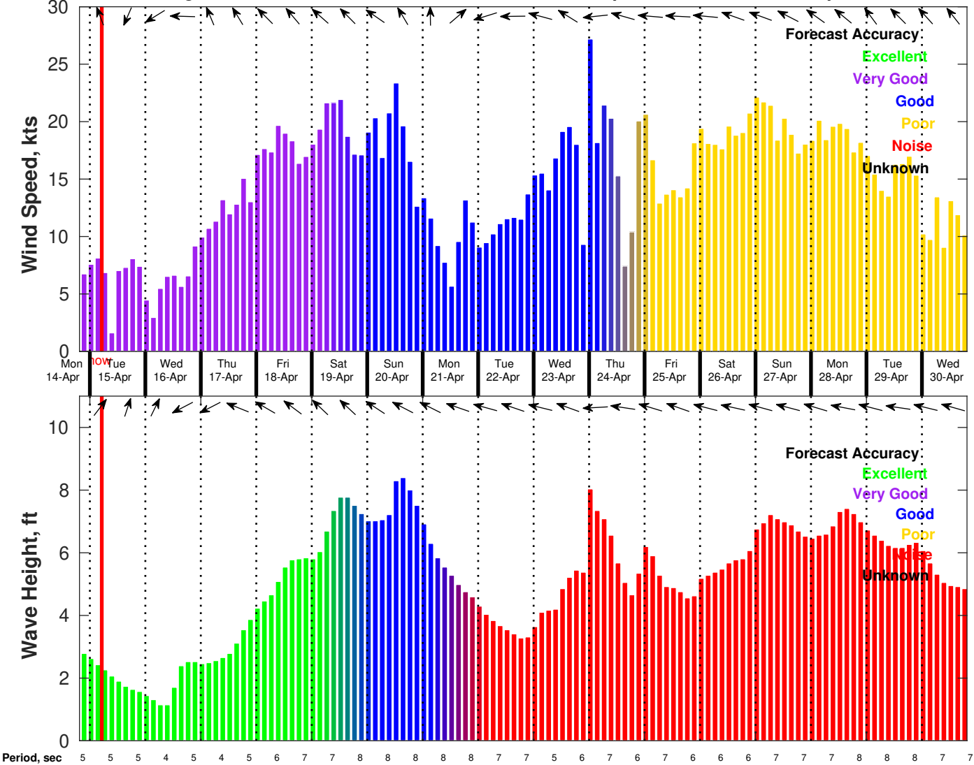
Wind & Wave Forecast for CTI Enbridge Kaskida & Tiber PPL Geotechnical from 14-Apr-2025 20:00:00 to 30-Apr-2025 20:00:00
