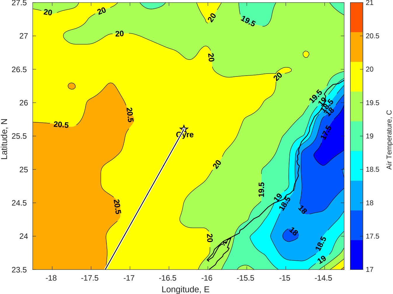
Air Temperature (C) for Gyre at 15-Apr-2025
