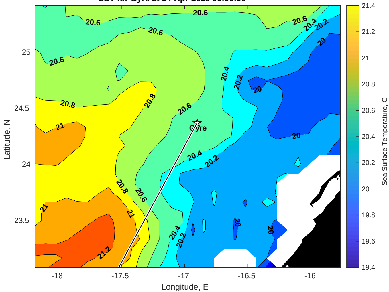
SST for Gyre at 14-Apr-2025 00:00:00
