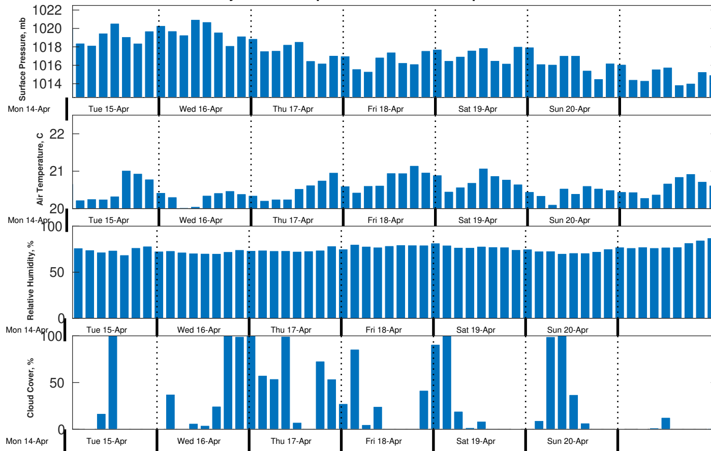
Met Forecast for Gyre from 14-Apr-2025 23:00:00 to 21-Apr-2025 23:00:00
