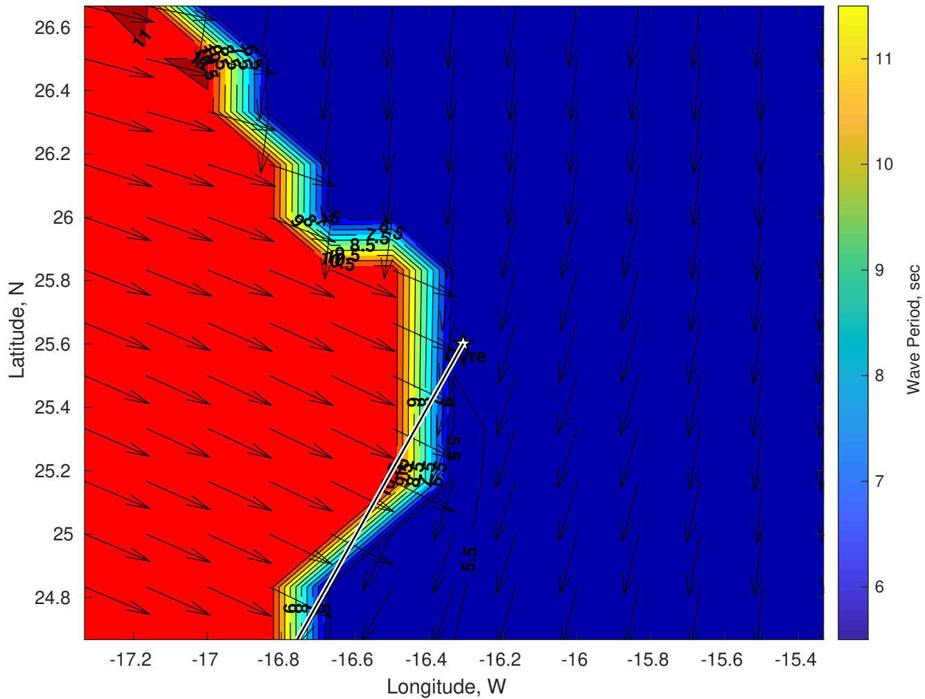
Wave Period (sec) for Gyre at 15-Apr-2025 09:00:00
