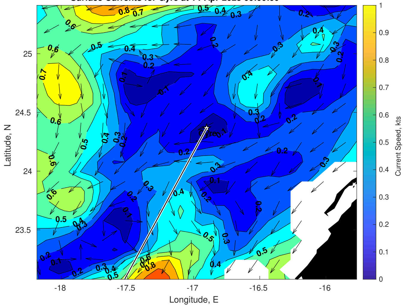
Surface Currents for Gyre at 14-Apr-2025 00:00:00
