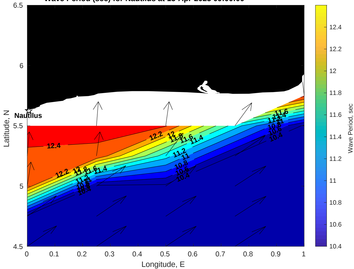
Wave Period (sec) for Nautilus at 15-Apr-2025 09:00:00
