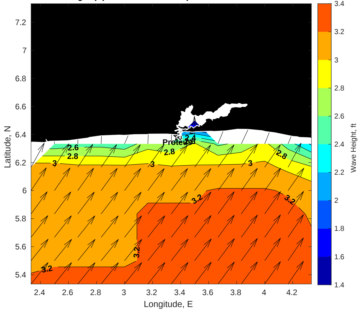
Wave Height (ft) for Proteus at 15-Apr-2025 09:00:00
