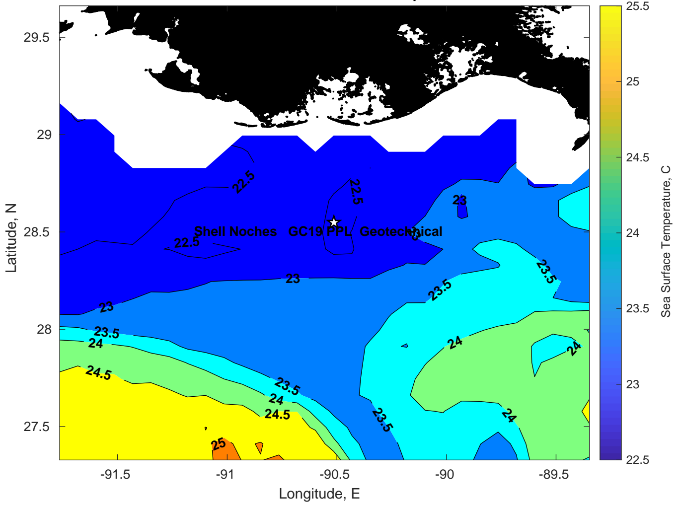
SST for Shell Noches GC19 PPL Geotechnical at 14-Apr-2025 00:00:00
