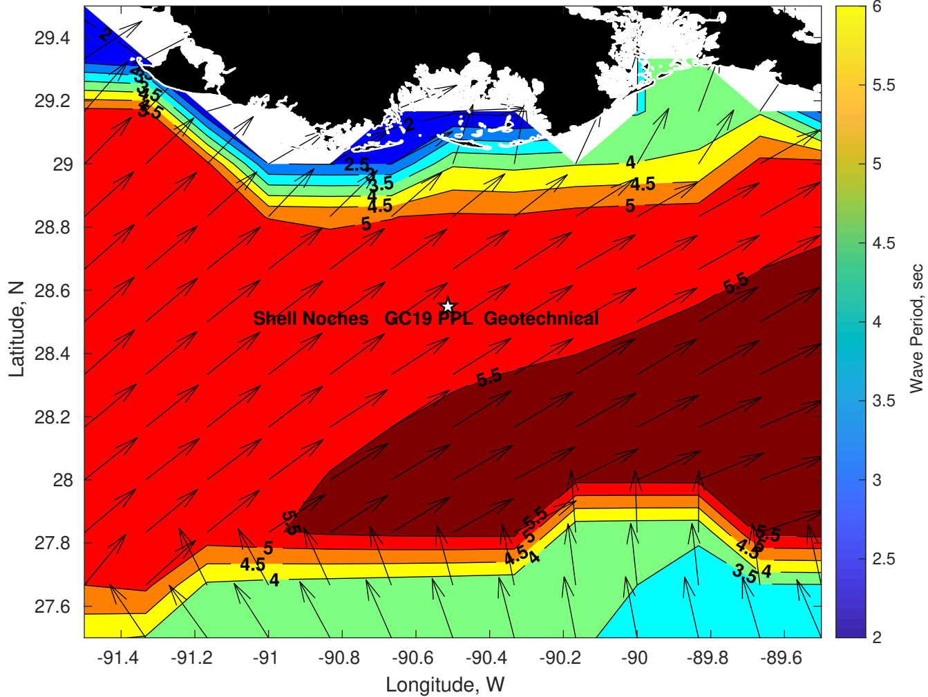
Wave Period (sec) for Shell Noches GC19 PPL Geotechnical at 15-Apr-2025 09:00:00
