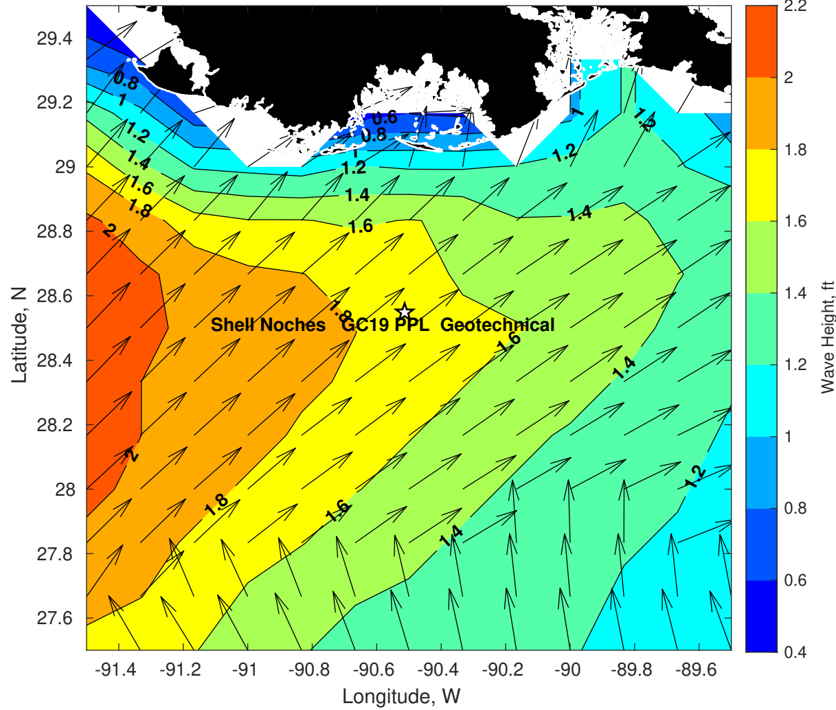
Wave Height (ft) for Shell Noches GC19 PPL Geotechnical at 15-Apr-2025 09:00:00
