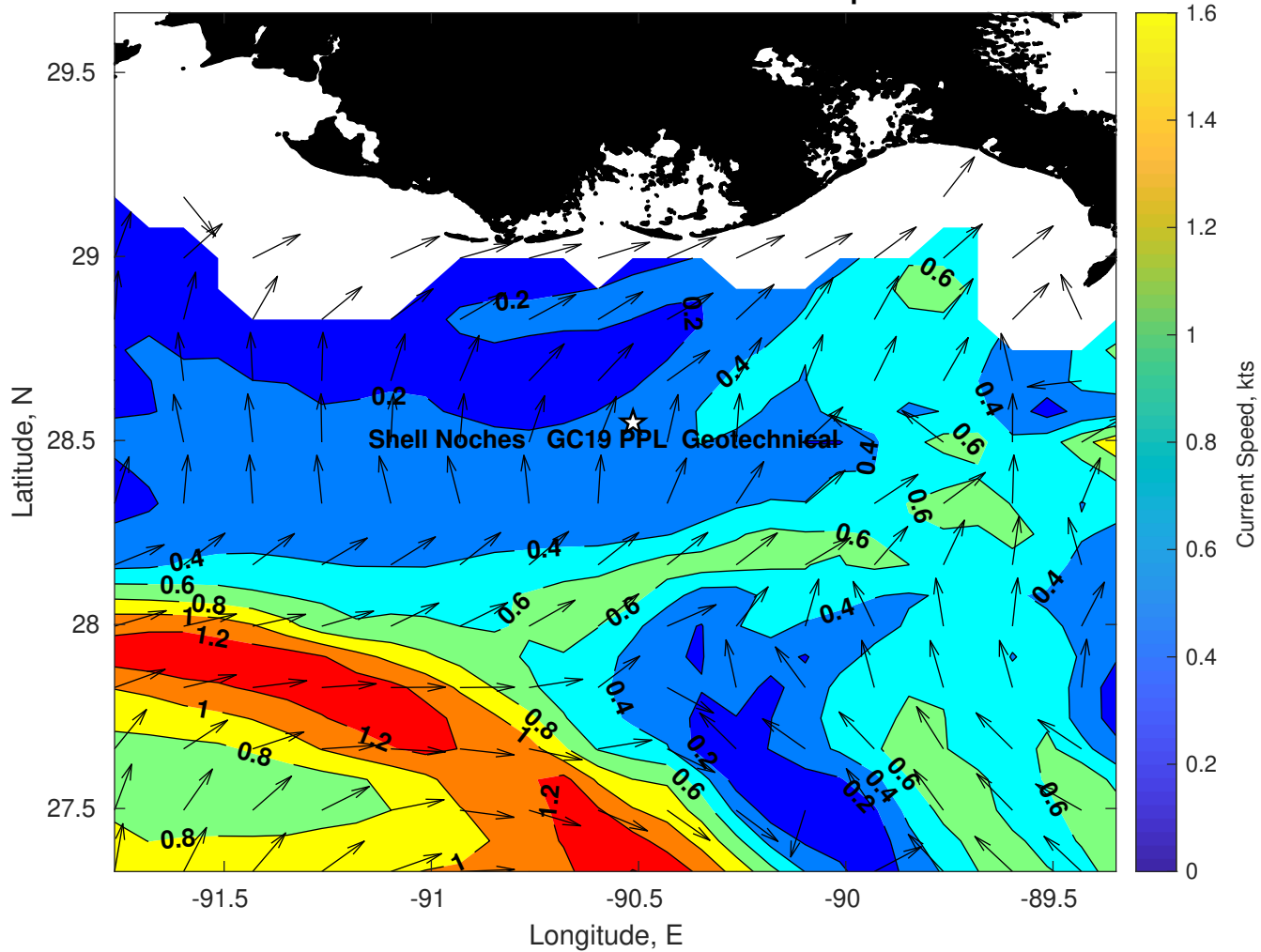
Surface Currents for Shell Noches GC19 PPL Geotechnical at 14-Apr-2025 00:00:00
