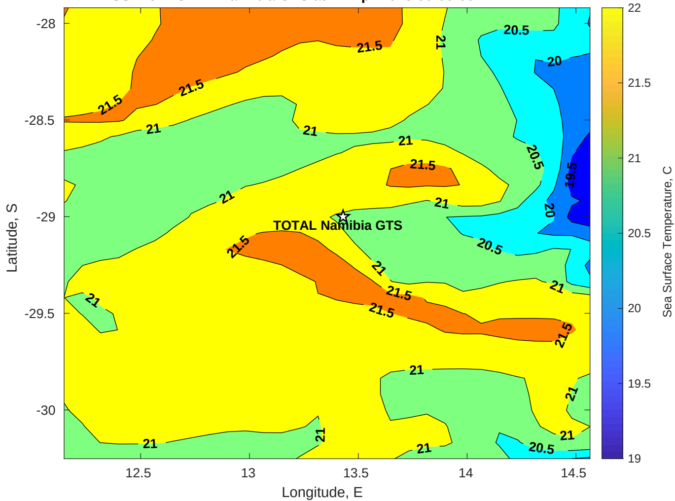
SST for TOTAL Namibia GTS at 14-Apr-2025 00:00:00
